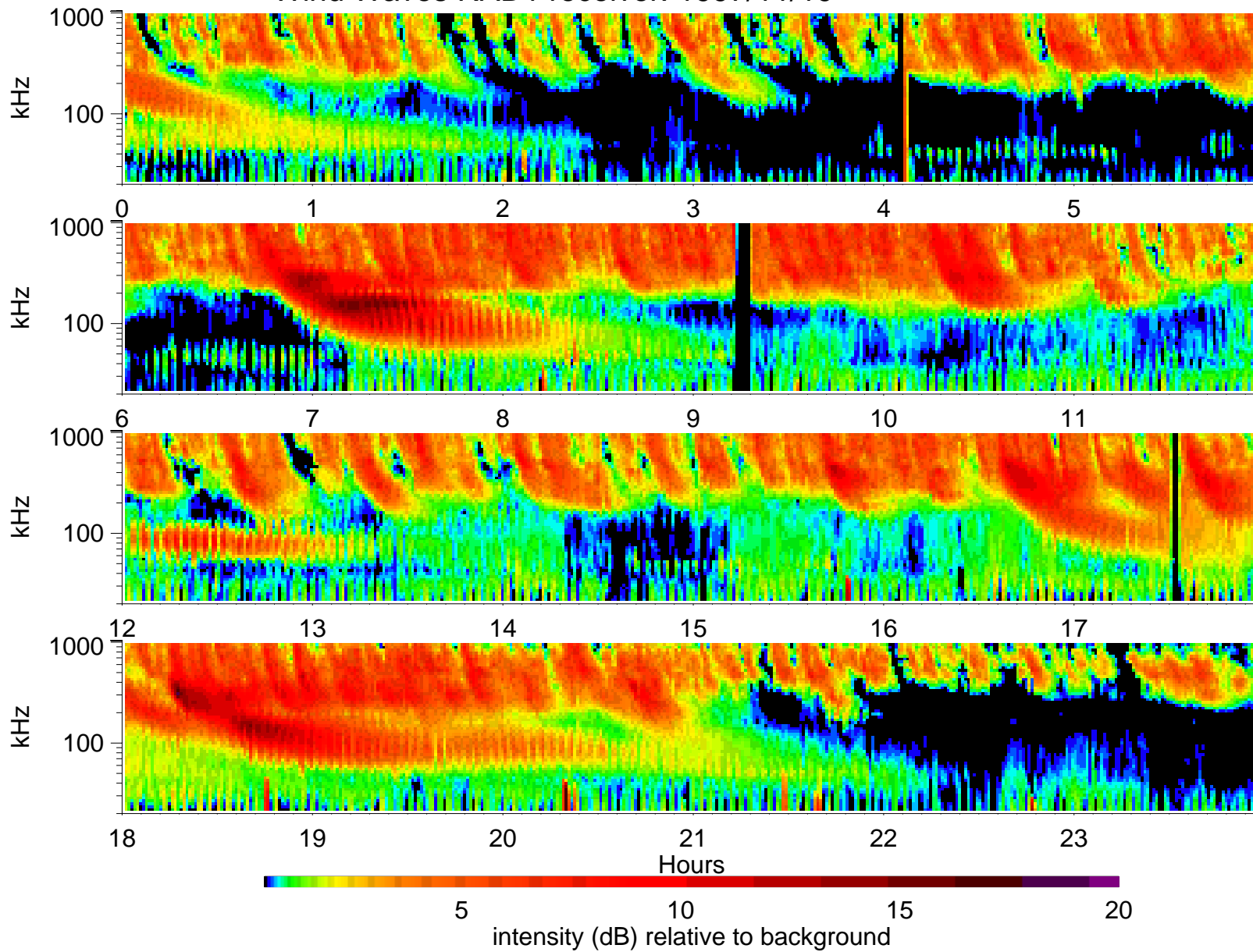
Wind Waves RAD1 receiver: 1997/11/19
