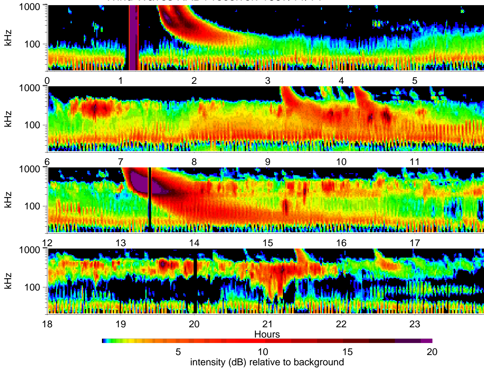
Wind Waves RAD1 receiver: 1997/11/14
