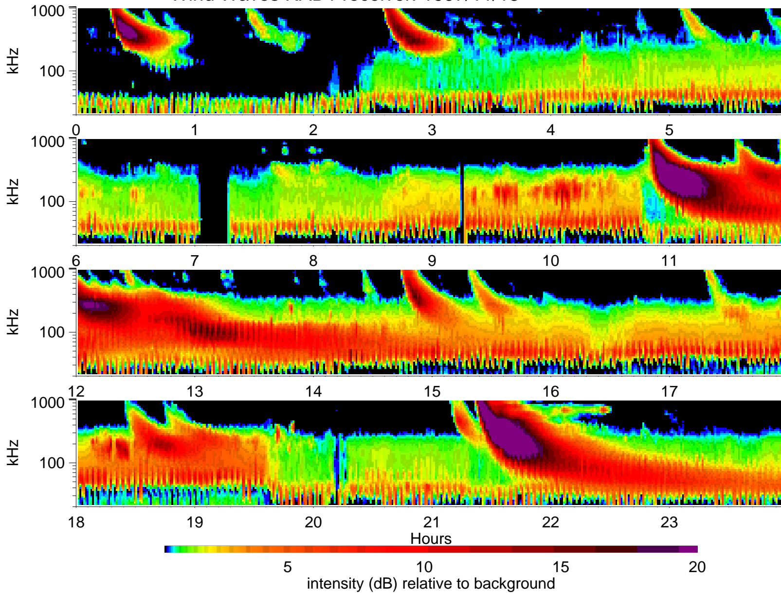
Wind Waves RAD1 receiver: 1997/11/13
