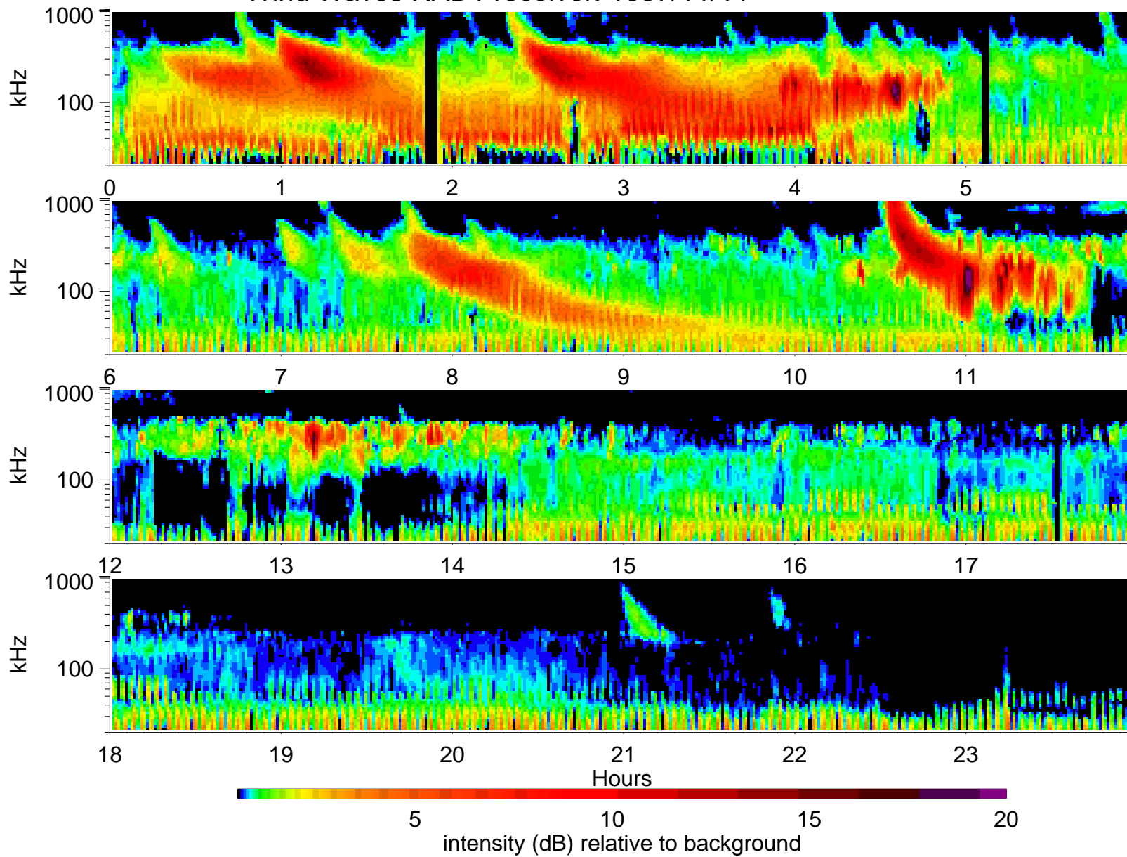
Wind Waves RAD1 receiver: 1997/11/11
