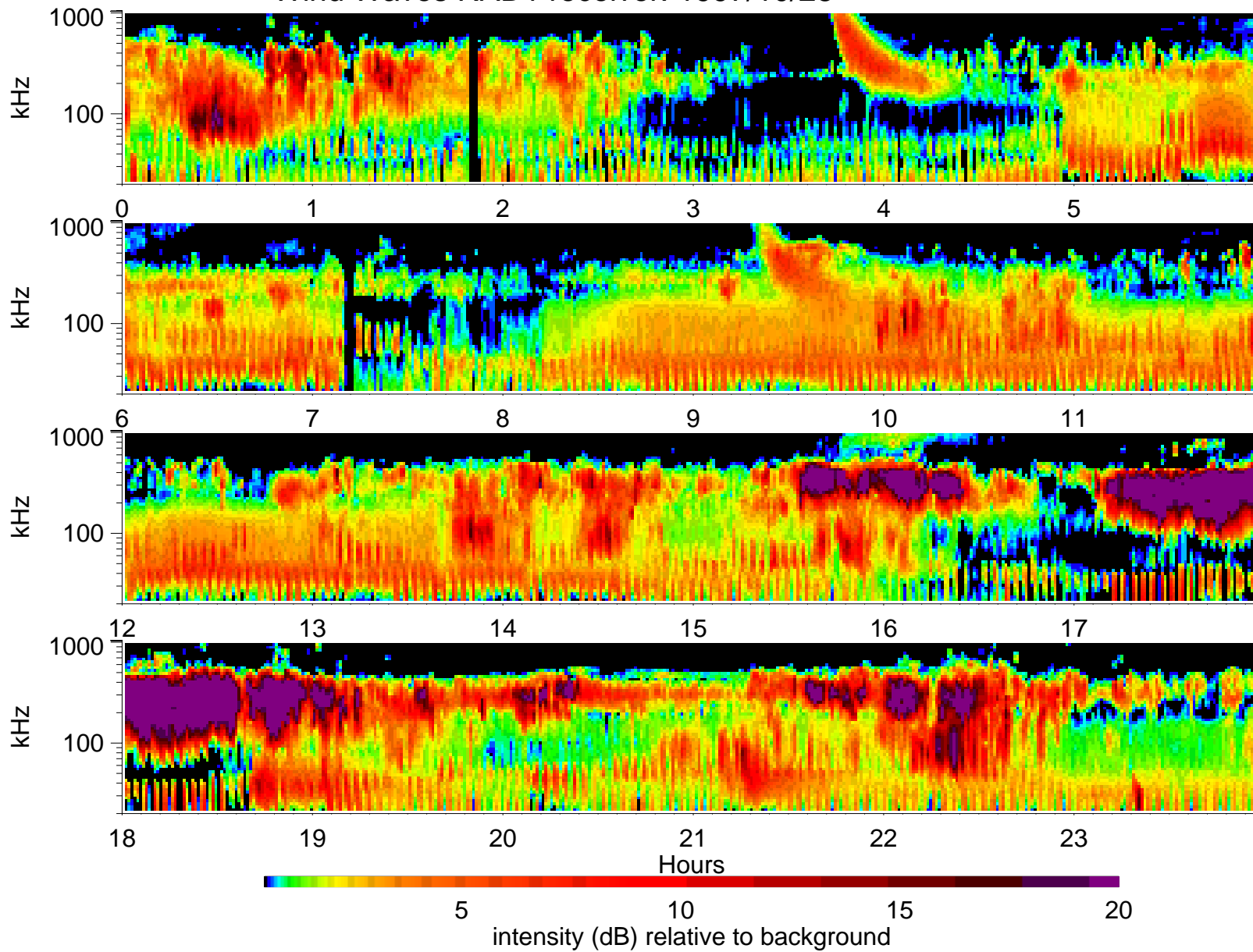
Wind Waves RAD1 receiver: 1997/10/28
