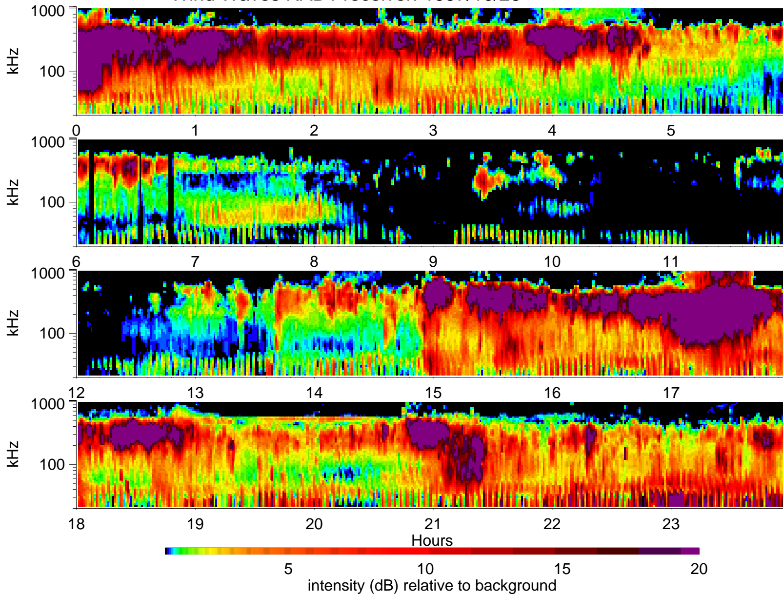
Wind Waves RAD1 receiver: 1997/10/26
