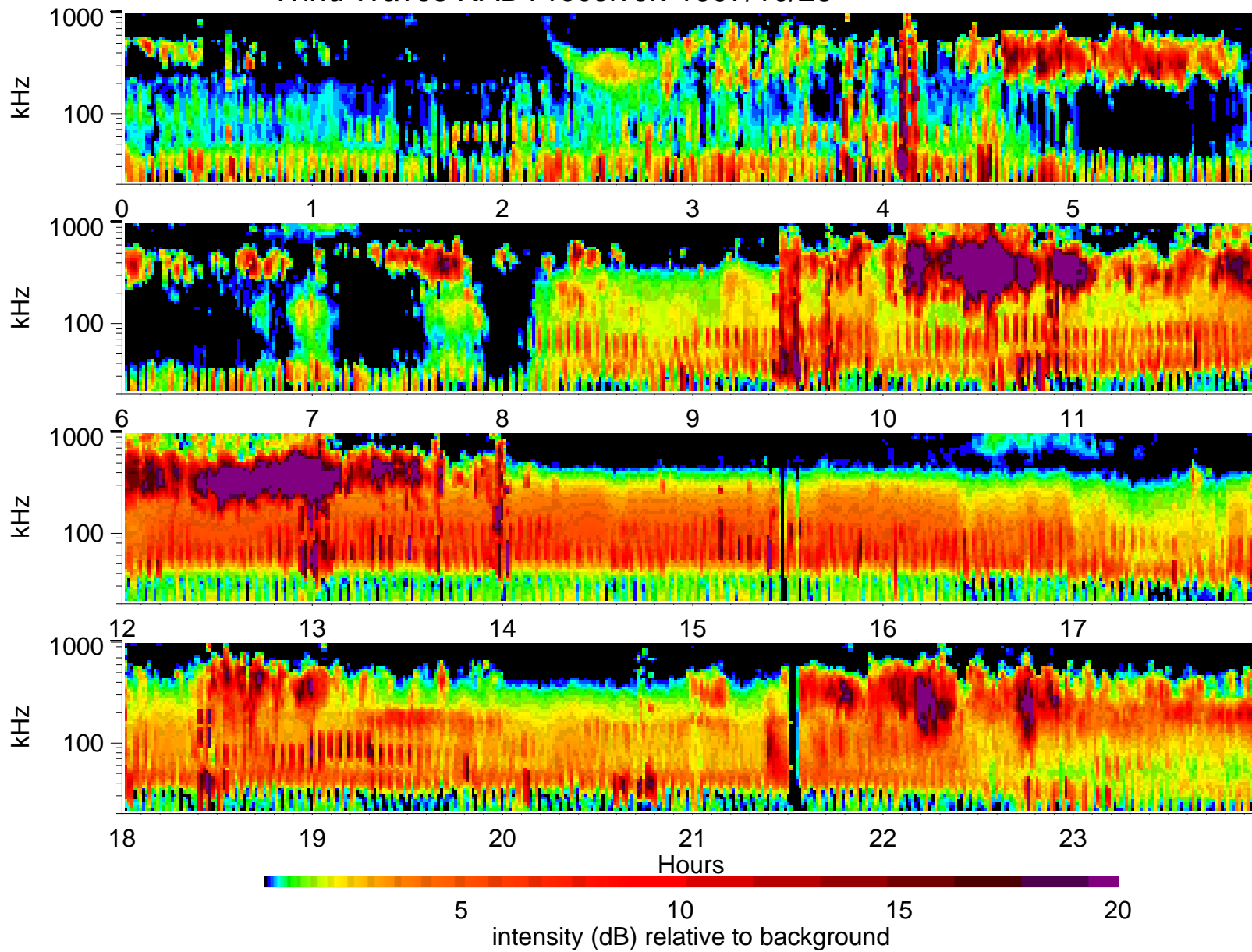
Wind Waves RAD1 receiver: 1997/10/23
