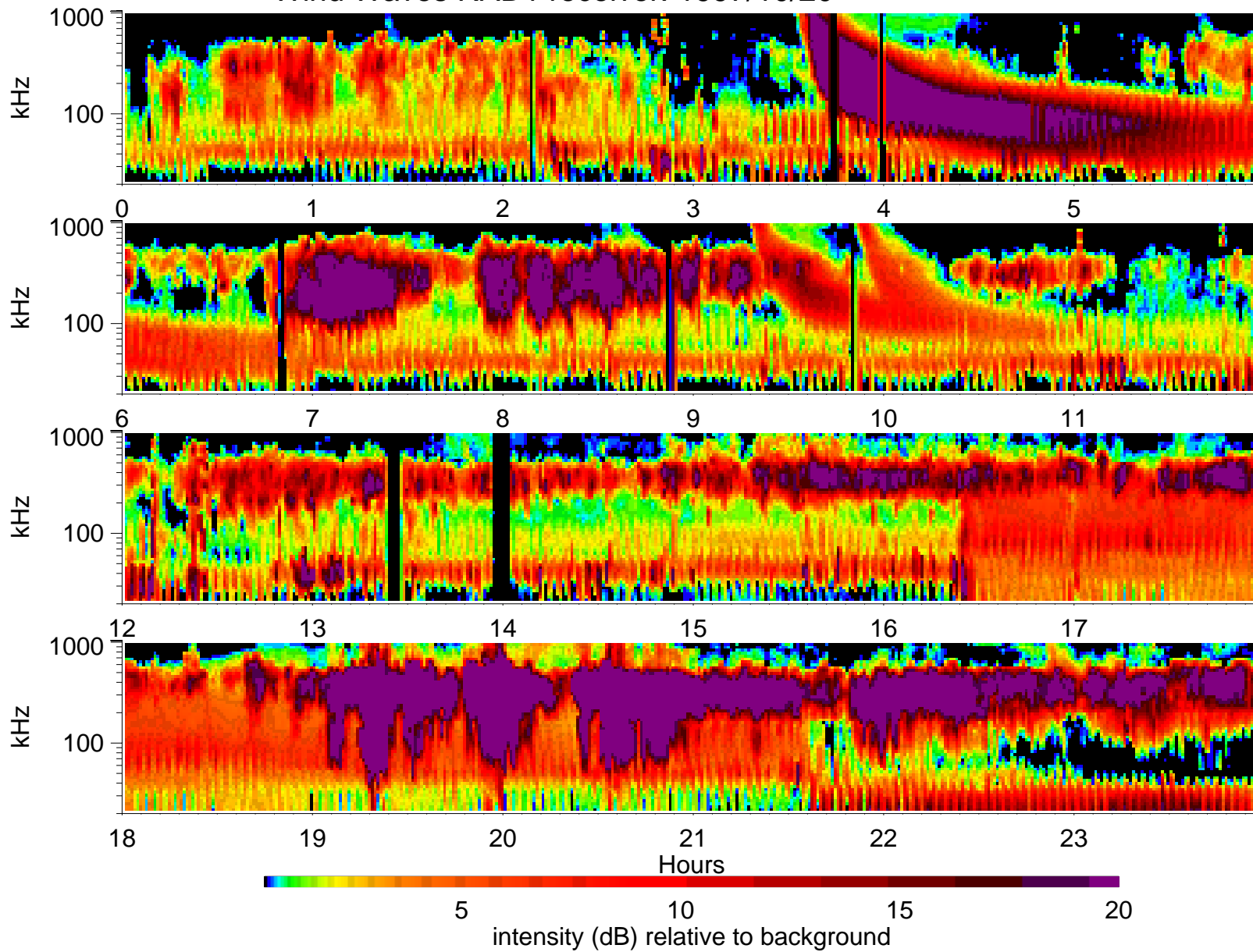
Wind Waves RAD1 receiver: 1997/10/20
