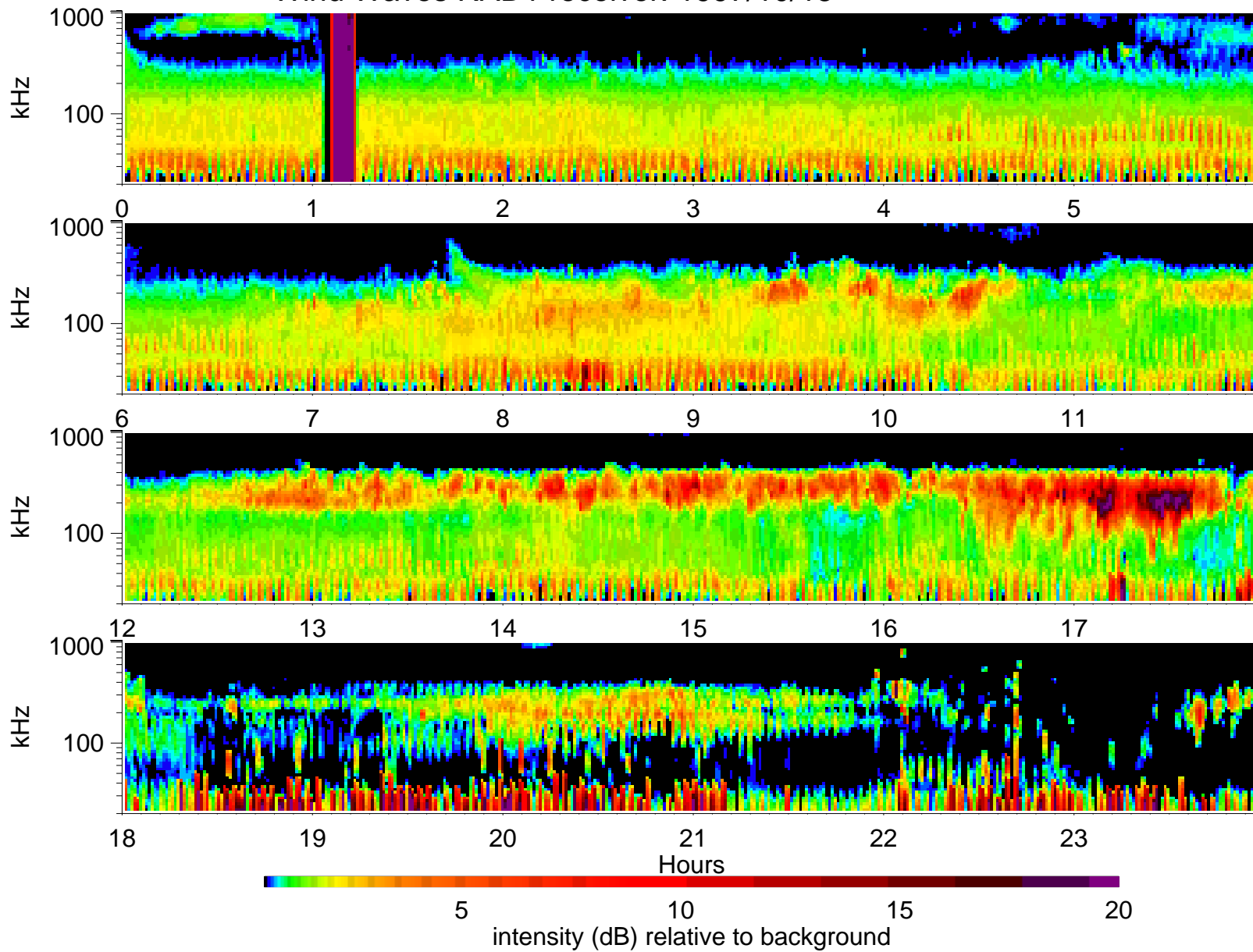
Wind Waves RAD1 receiver: 1997/10/15
