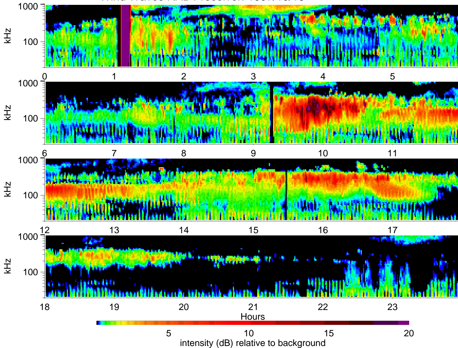
Wind Waves RAD1 receiver: 1997/10/13
