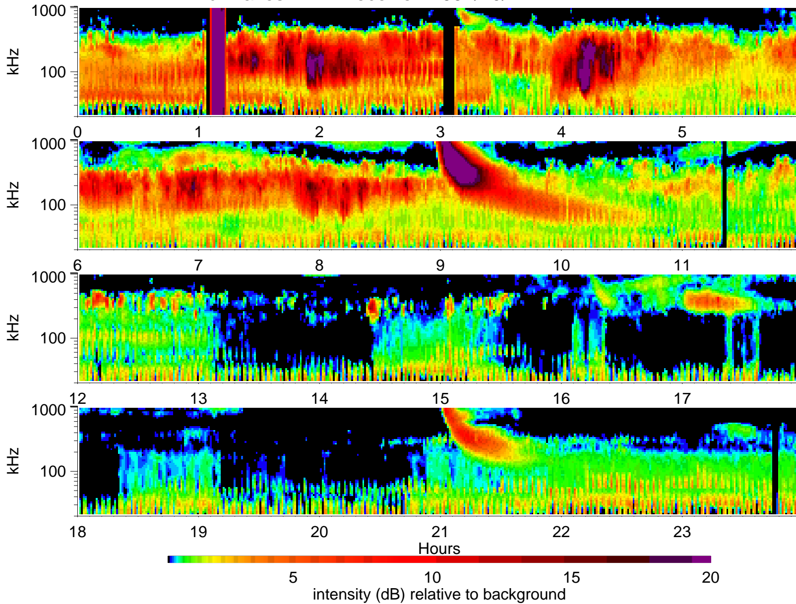
Wind Waves RAD1 receiver: 1997/10/11
