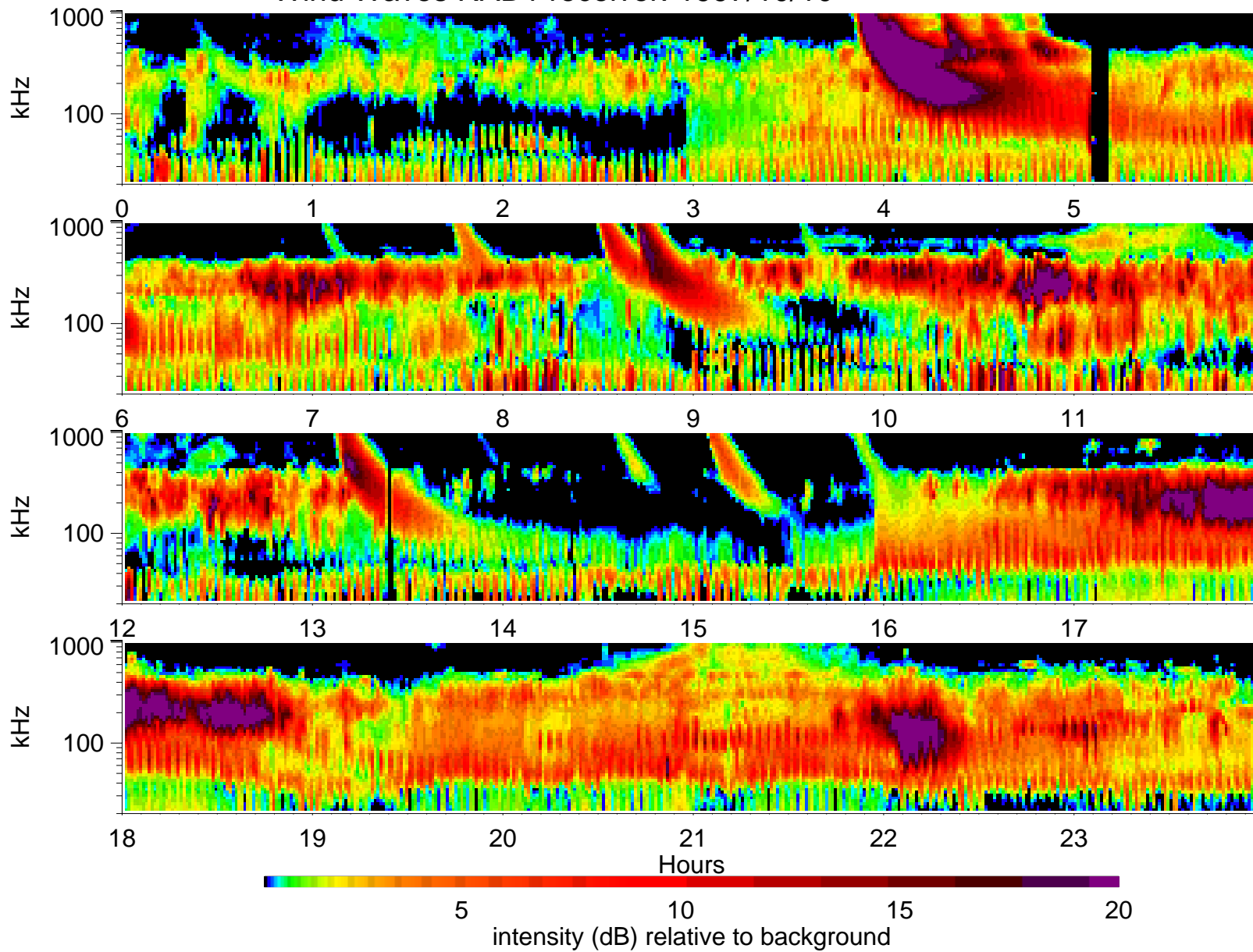
Wind Waves RAD1 receiver: 1997/10/10
