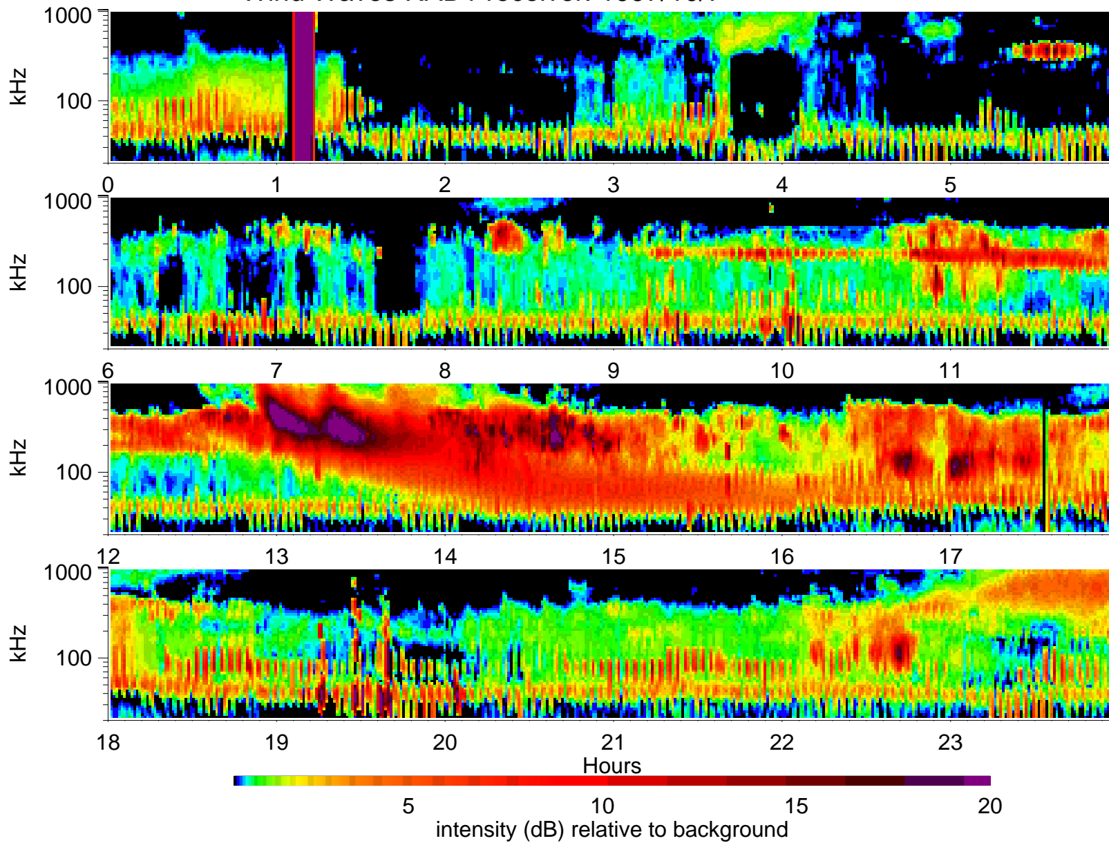
Wind Waves RAD1 receiver: 1997/10/7
