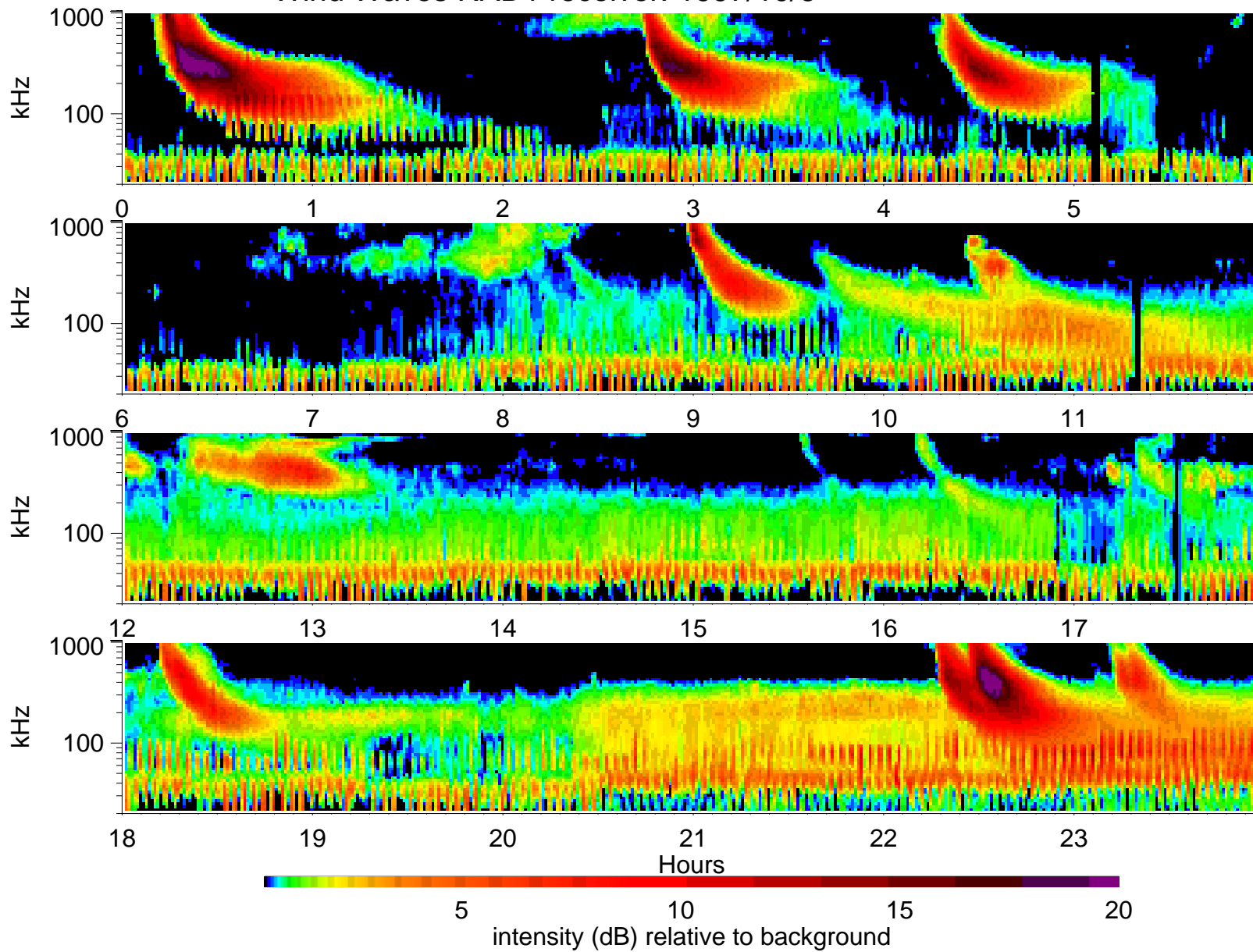
Wind Waves RAD1 receiver: 1997/10/6
