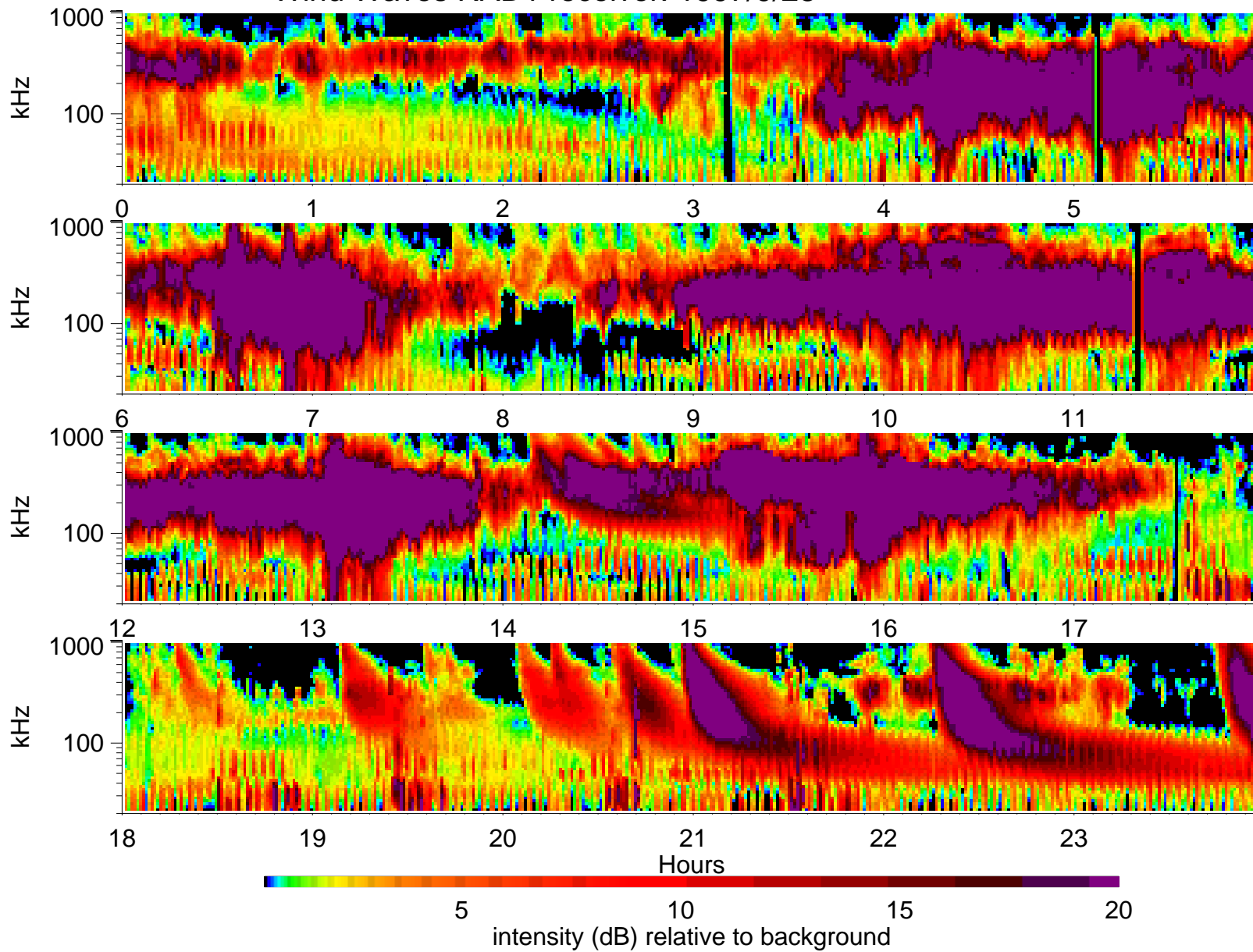
Wind Waves RAD1 receiver: 1997/9/28
