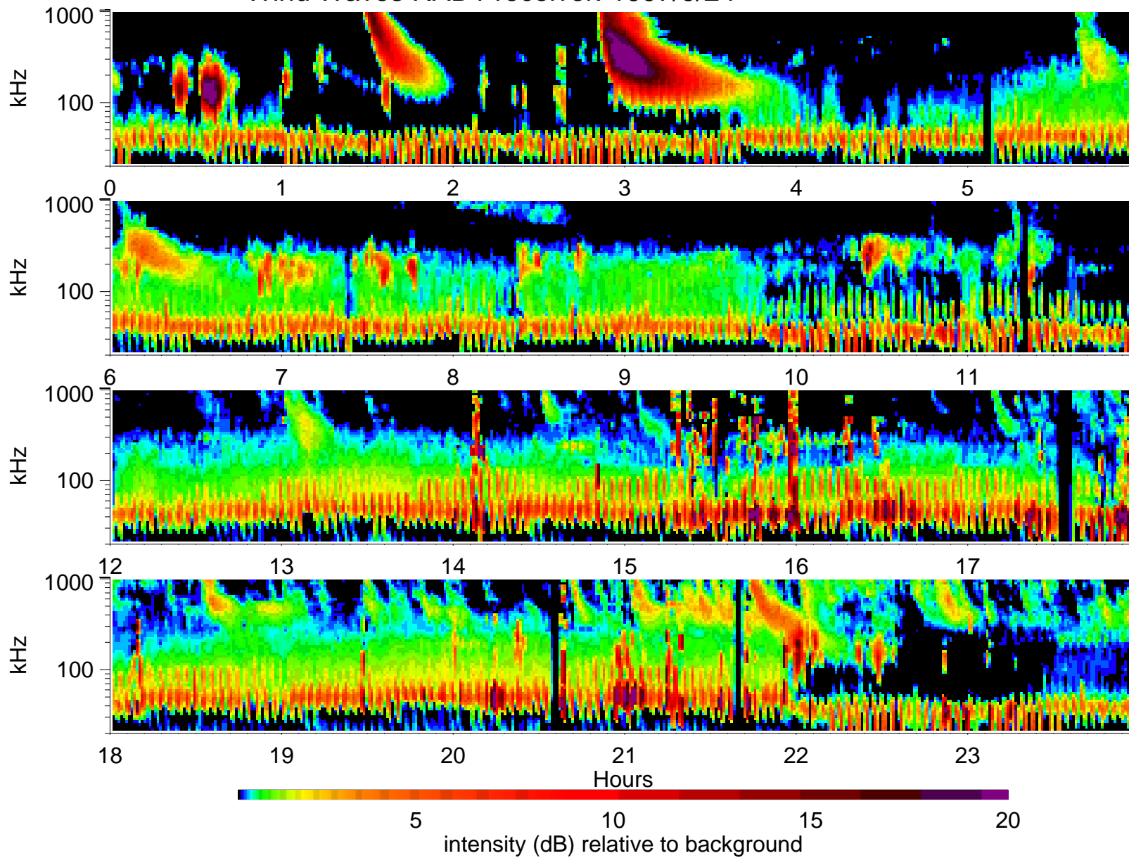
Wind Waves RAD1 receiver: 1997/9/24
