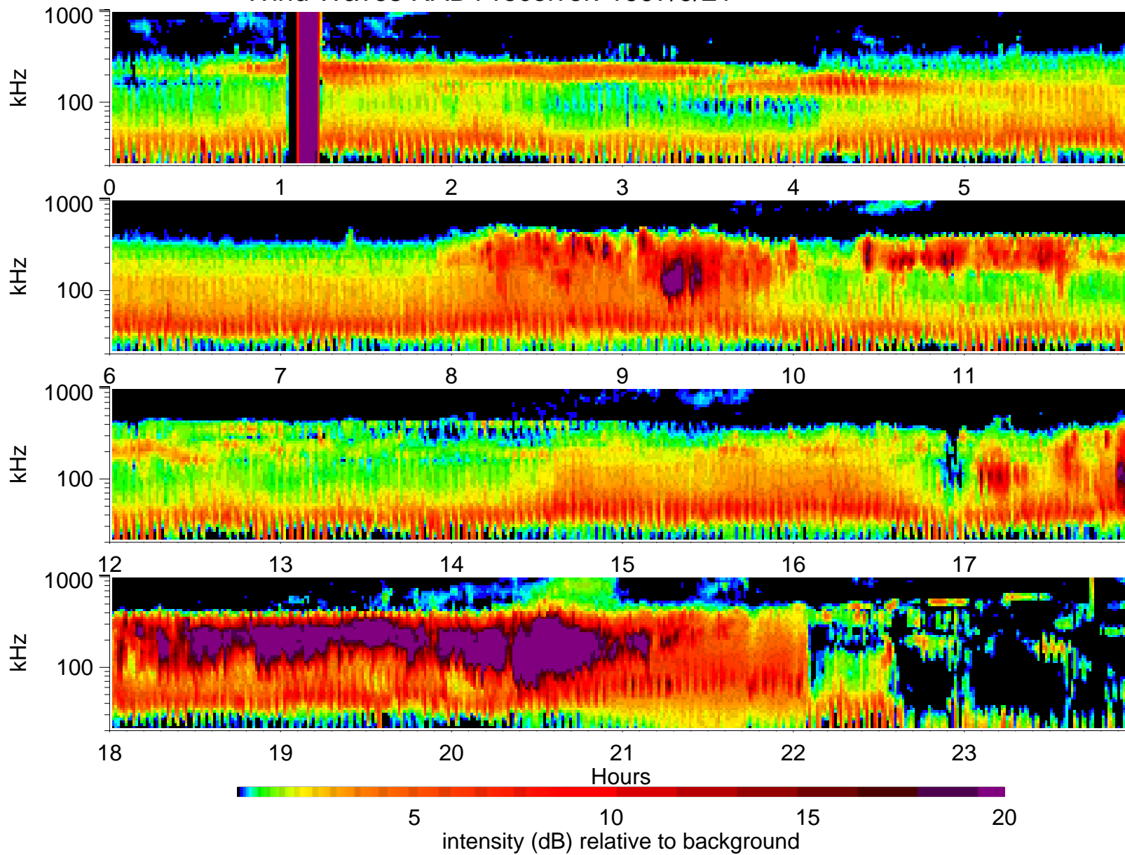
Wind Waves RAD1 receiver: 1997/9/21
