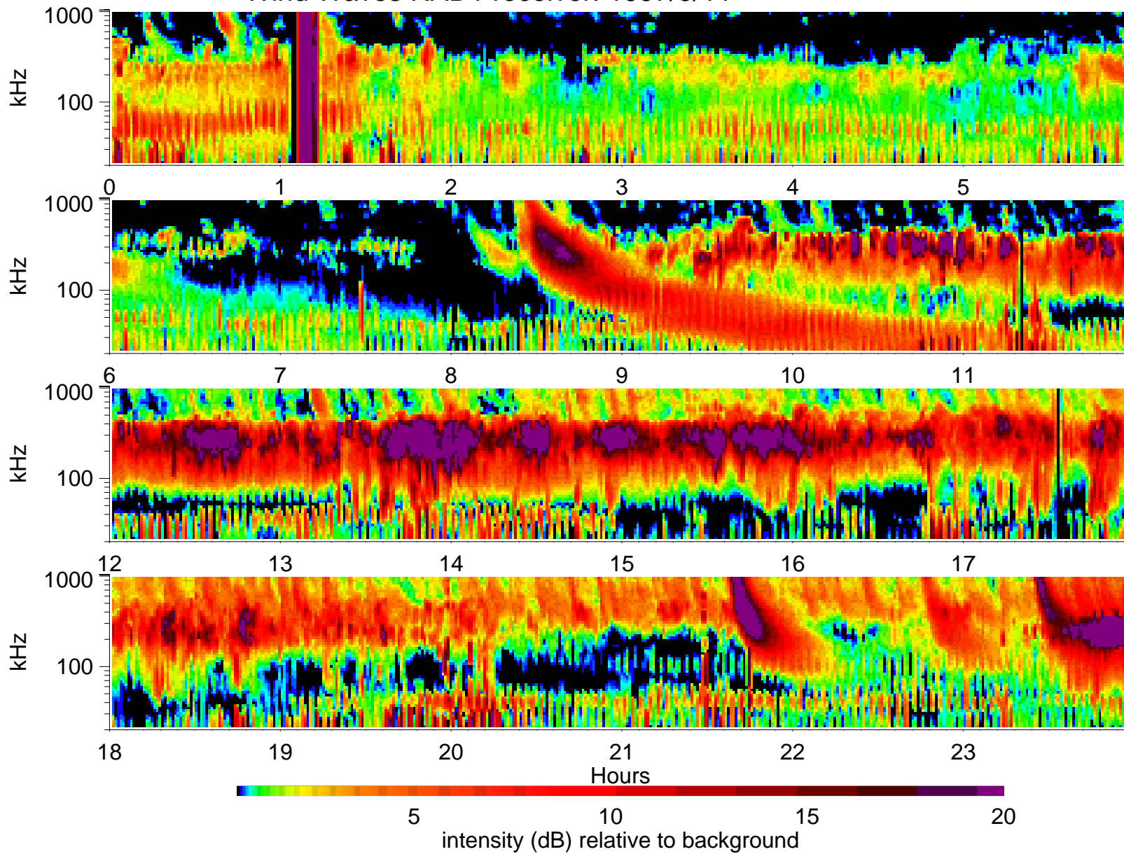
Wind Waves RAD1 receiver: 1997/9/11
