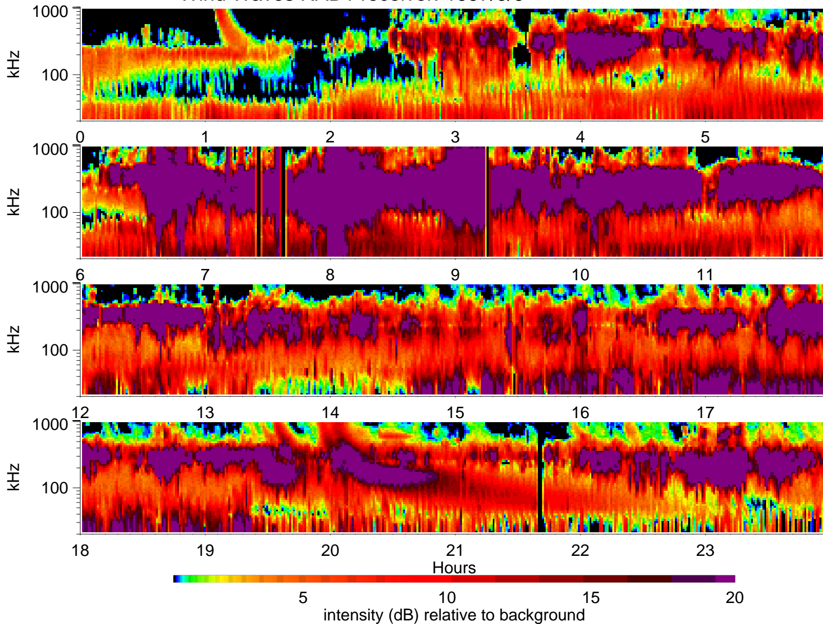
Wind Waves RAD1 receiver: 1997/9/9
