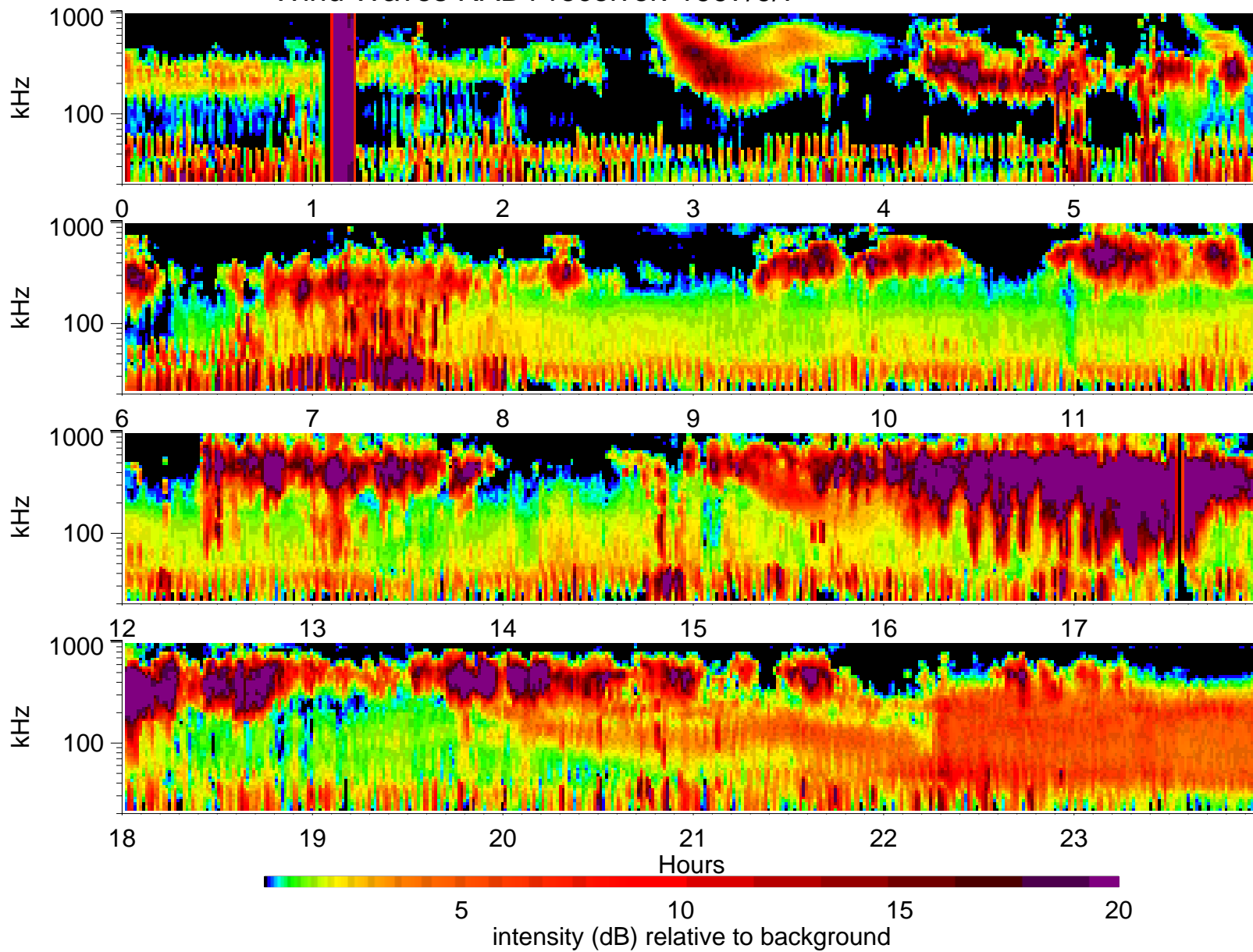
Wind Waves RAD1 receiver: 1997/9/7
