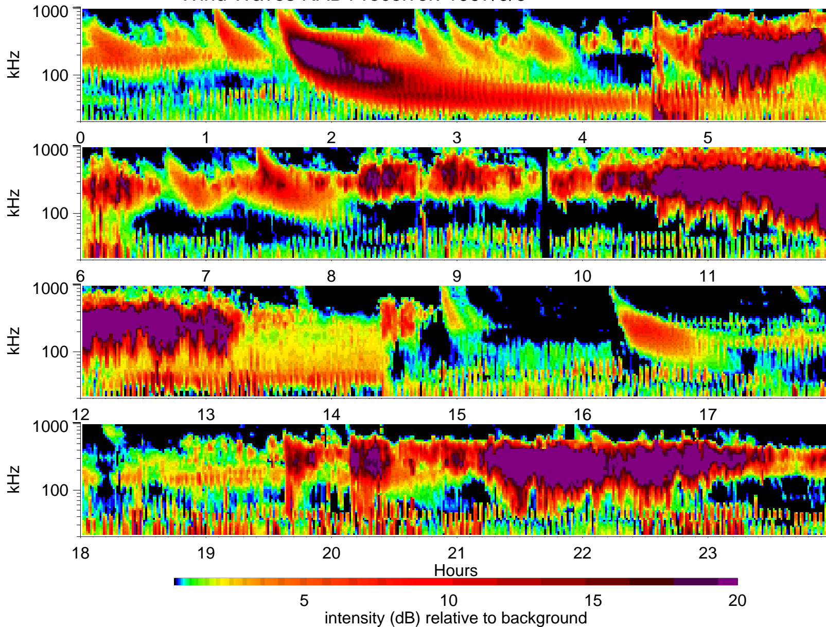
Wind Waves RAD1 receiver: 1997/9/6
