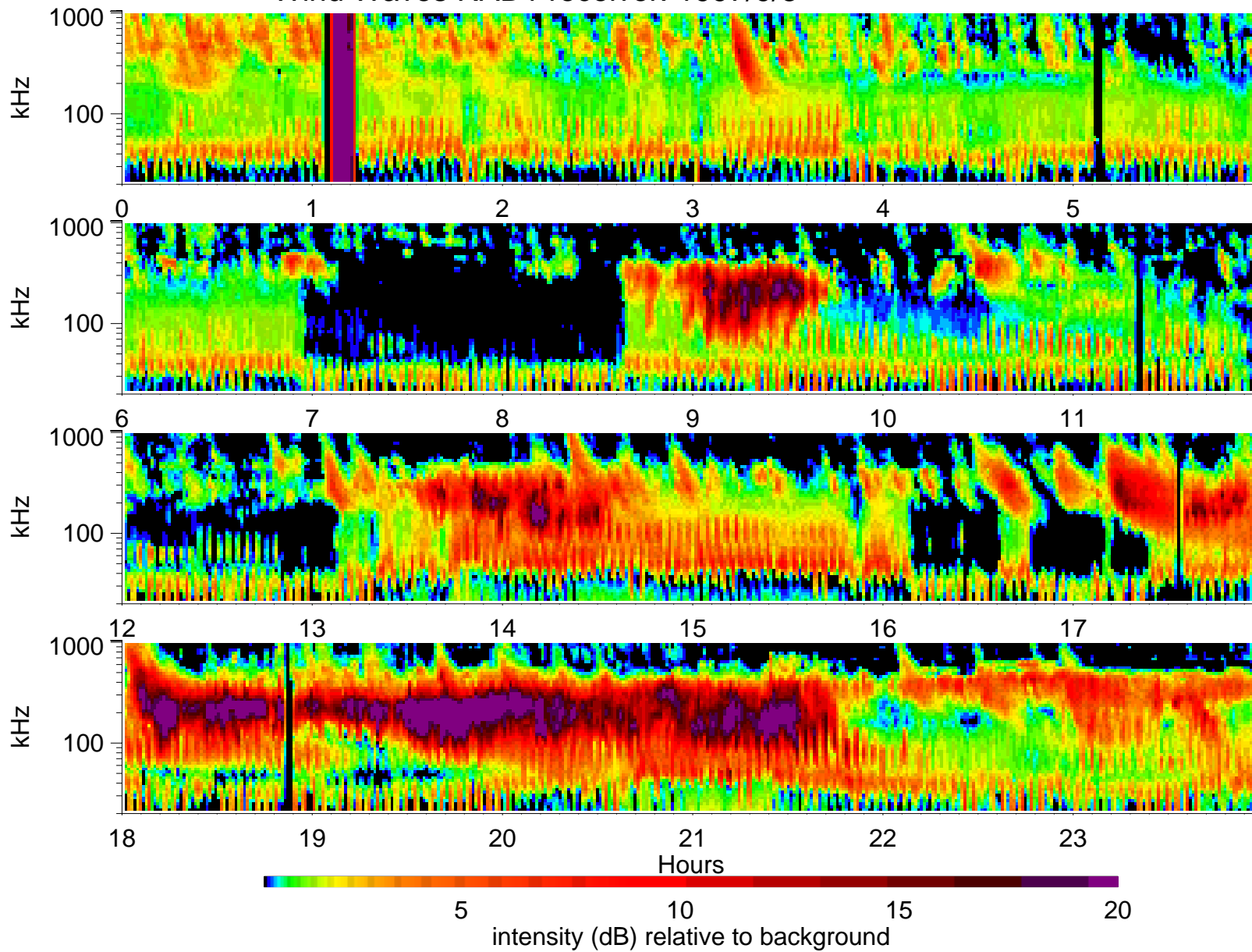
Wind Waves RAD1 receiver: 1997/9/3
