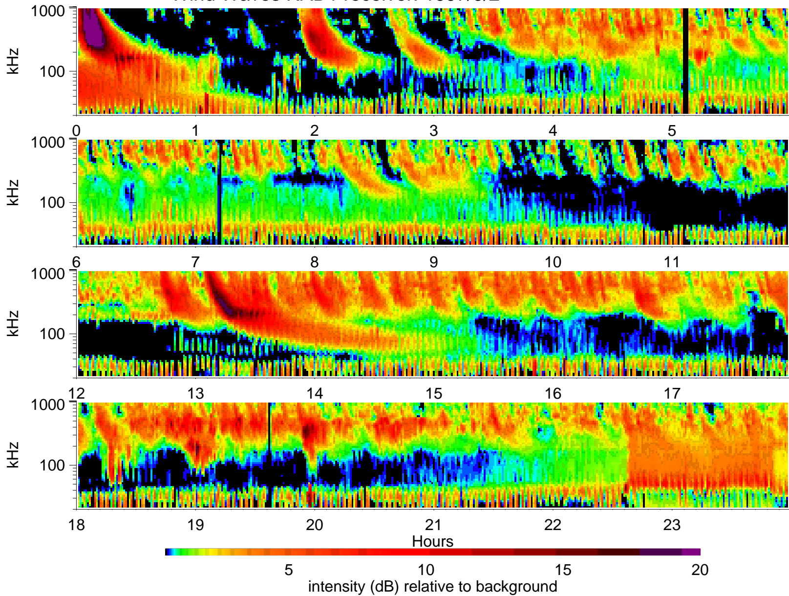
Wind Waves RAD1 receiver: 1997/9/2
