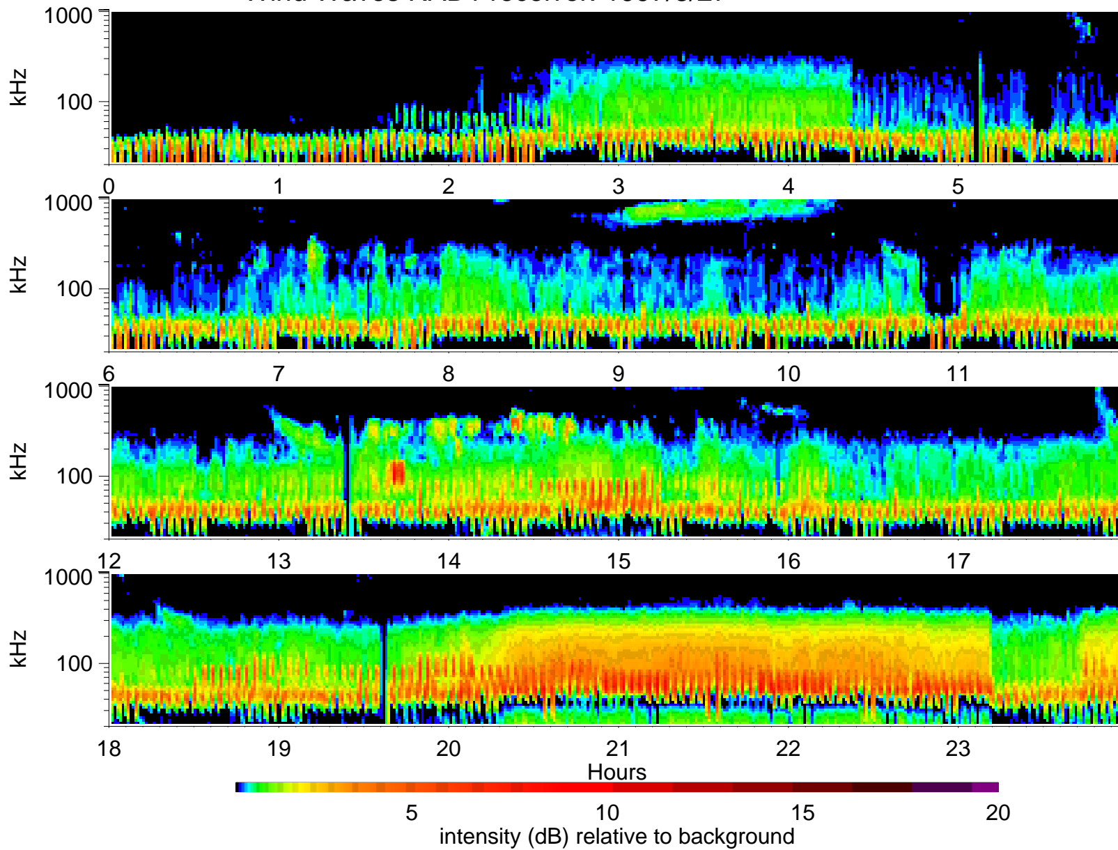
Wind Waves RAD1 receiver: 1997/8/27
