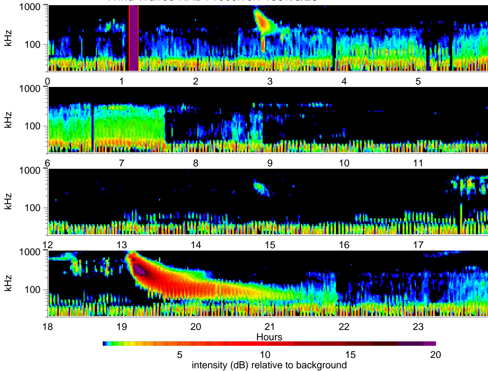
Wind Waves RAD1 receiver: 1997/8/26
