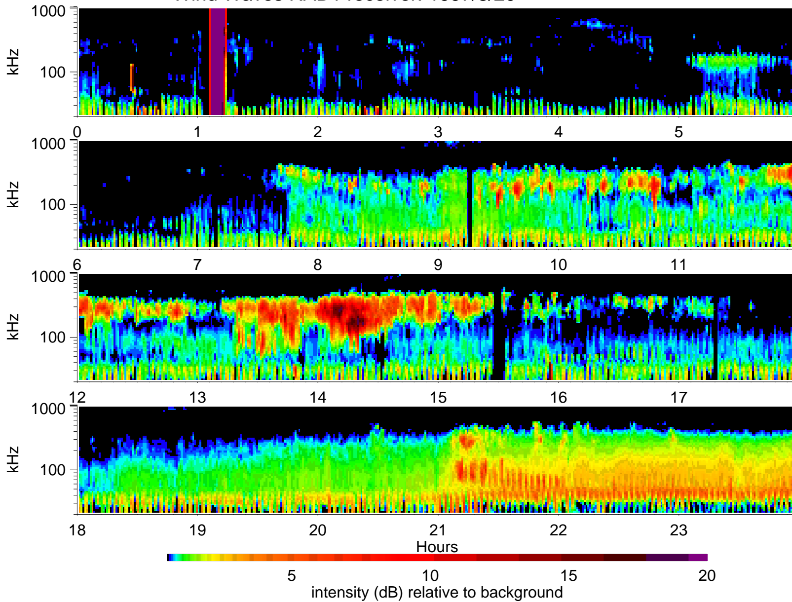
Wind Waves RAD1 receiver: 1997/8/20
