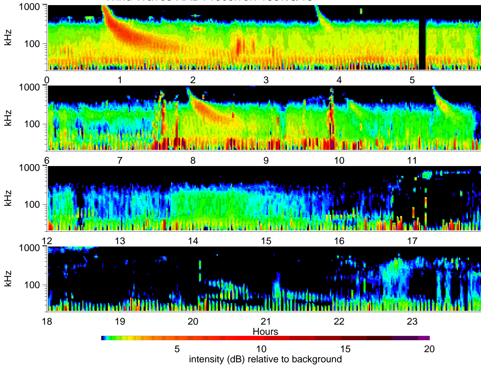
Wind Waves RAD1 receiver: 1997/8/19
