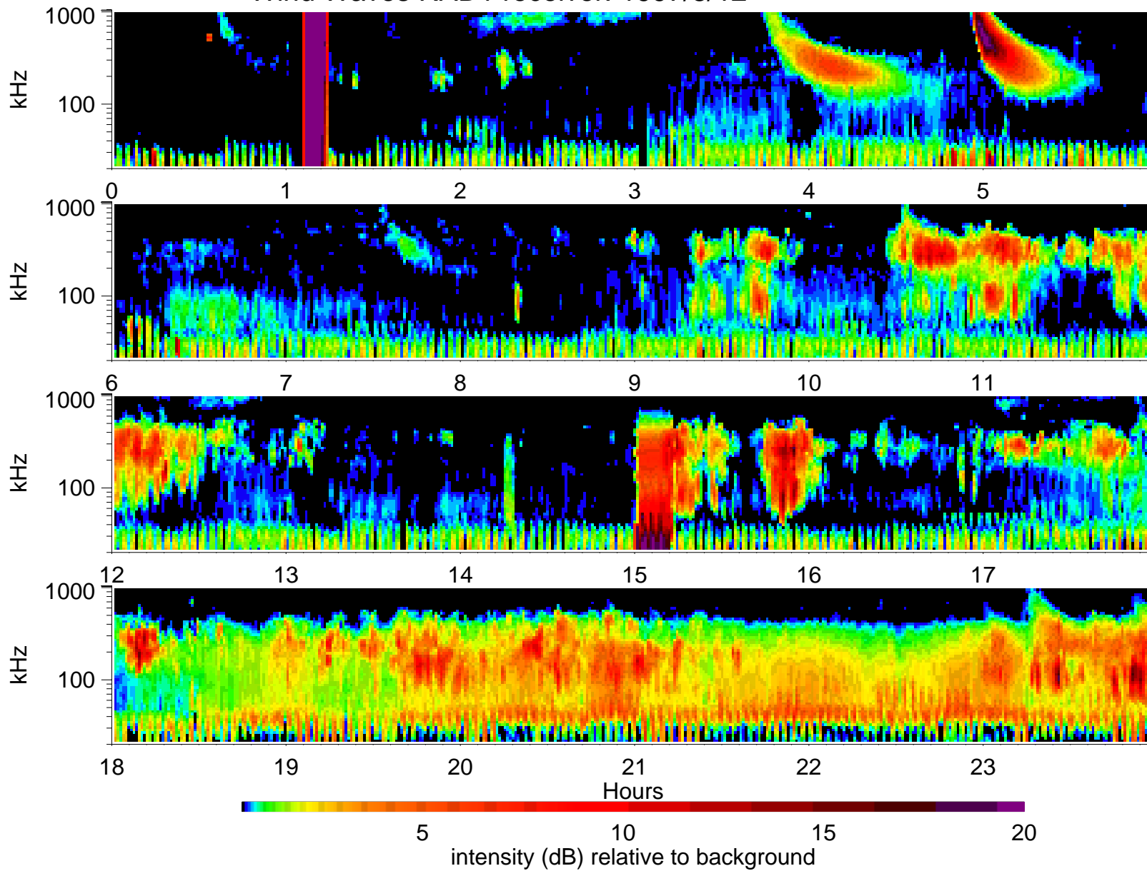
Wind Waves RAD1 receiver: 1997/8/12
