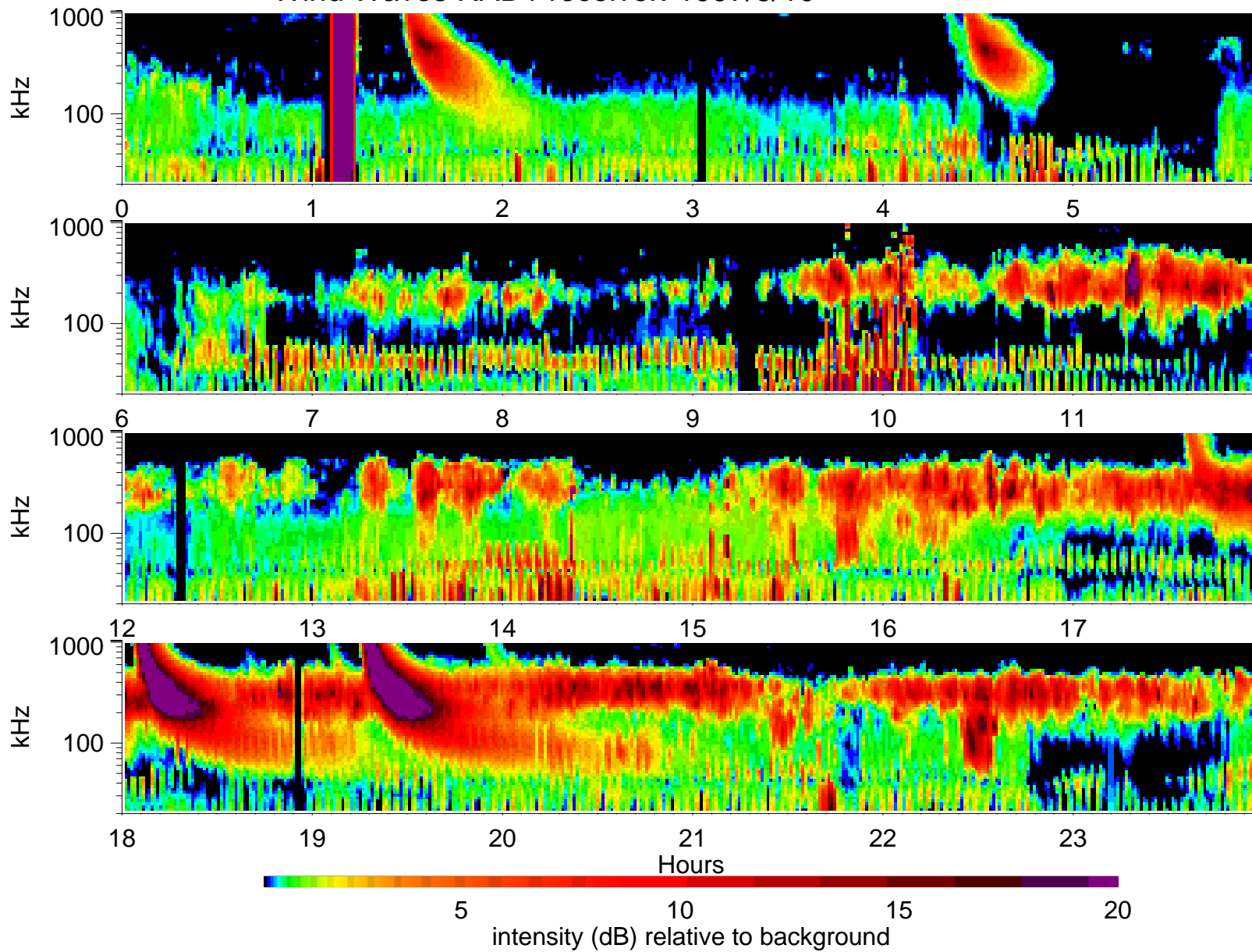
Wind Waves RAD1 receiver: 1997/8/10
