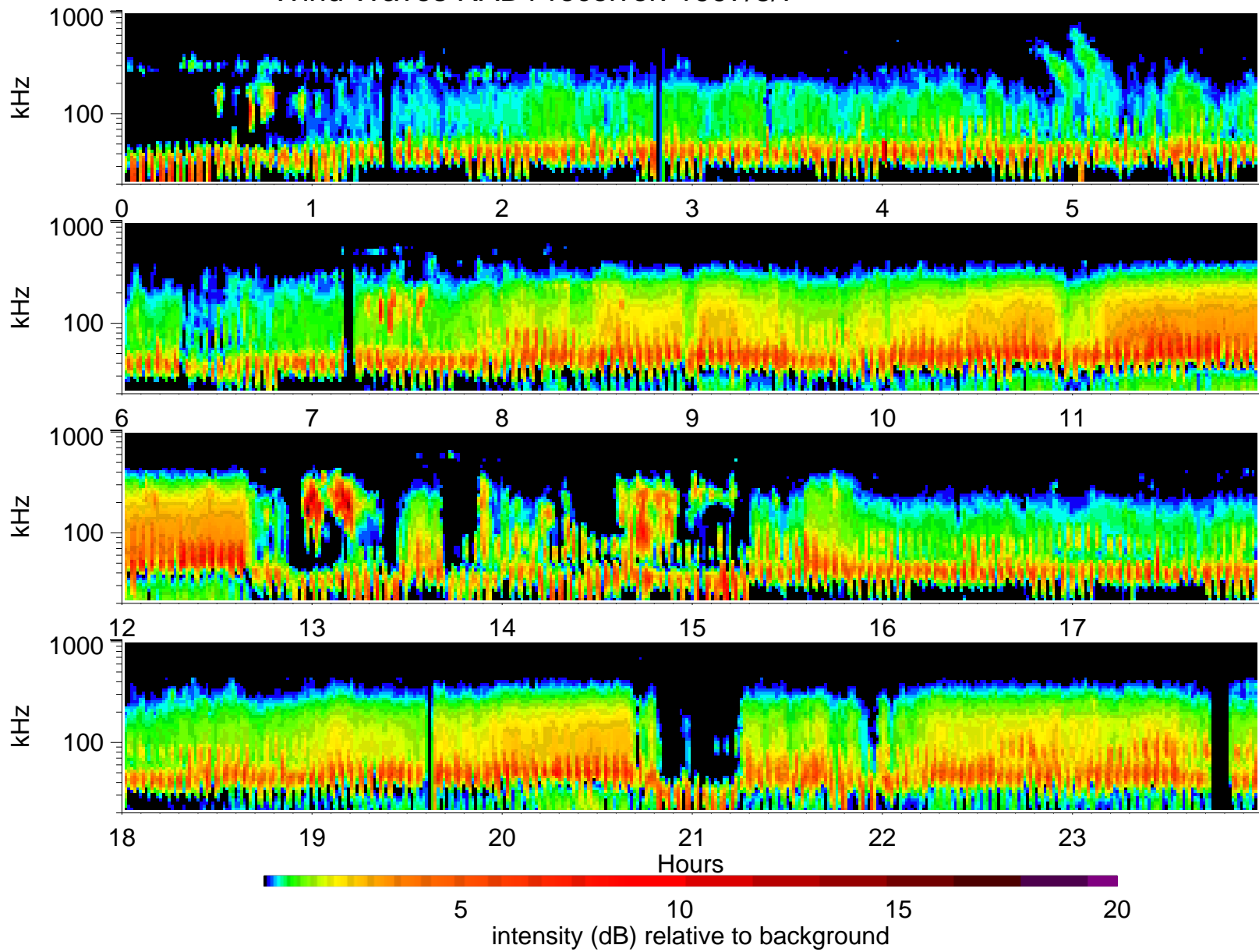
Wind Waves RAD1 receiver: 1997/8/7
