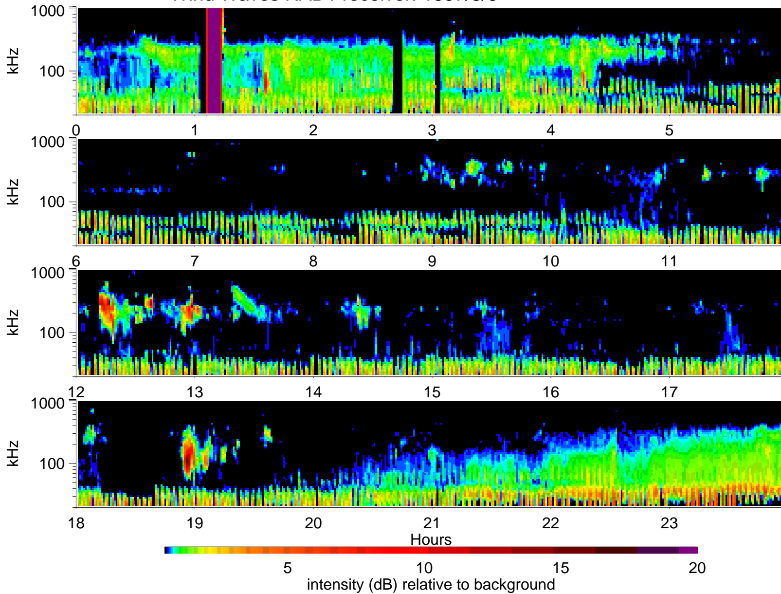
Wind Waves RAD1 receiver: 1997/8/6
