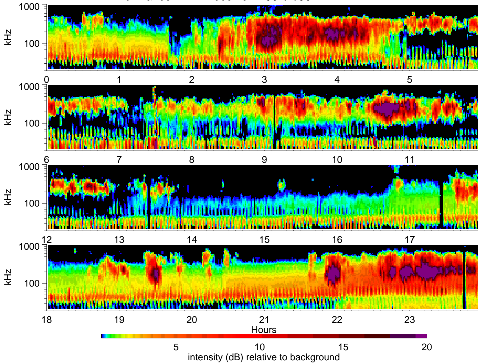
Wind Waves RAD1 receiver: 1997/7/30
