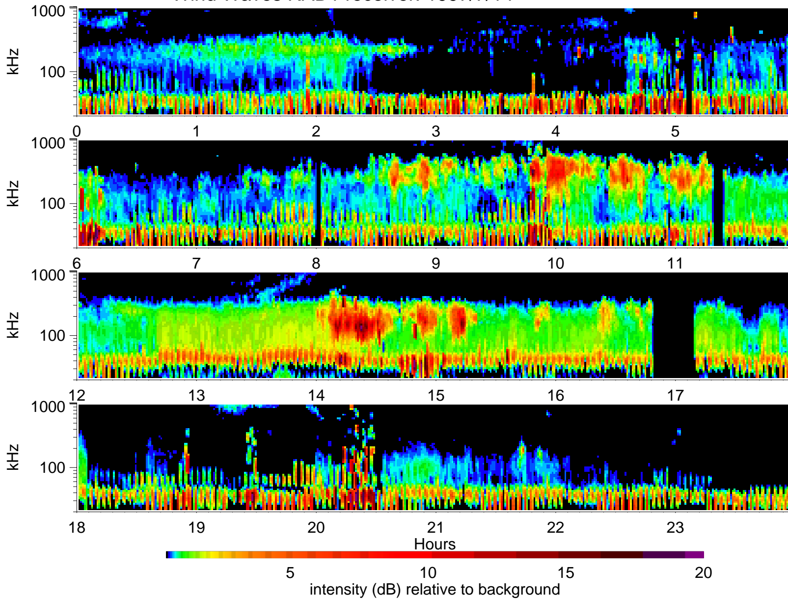
Wind Waves RAD1 receiver: 1997/7/14
