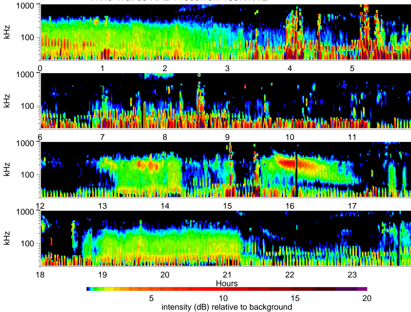
Wind Waves RAD1 receiver: 1997/7/12
