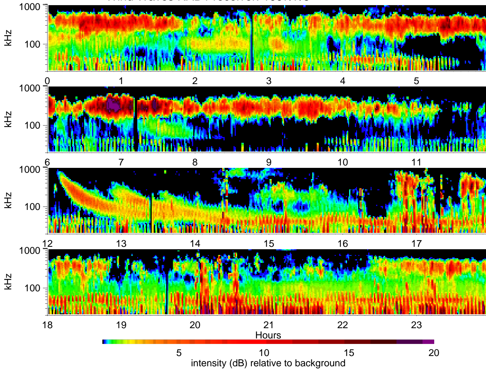
Wind Waves RAD1 receiver: 1997/7/8
