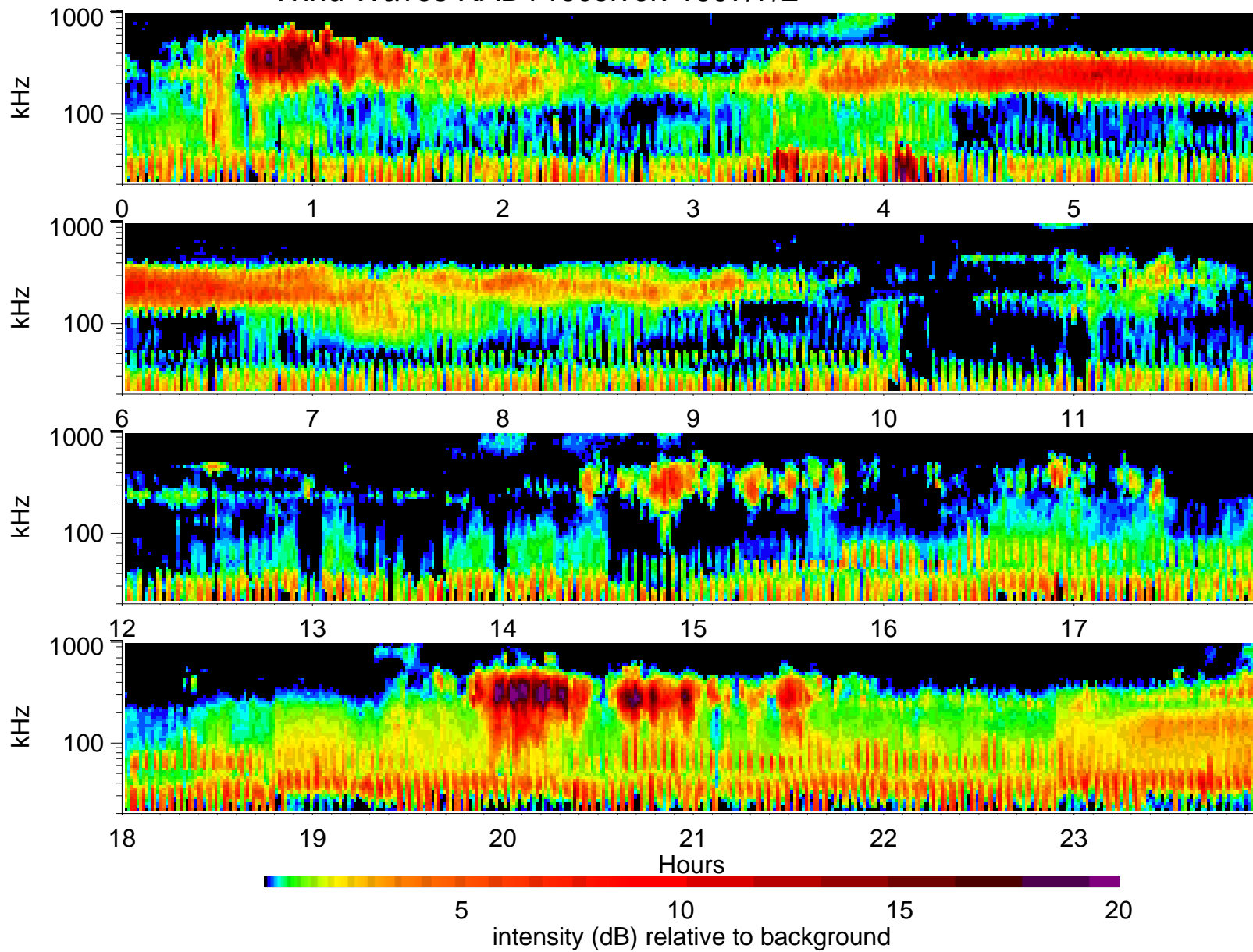
Wind Waves RAD1 receiver: 1997/7/2
