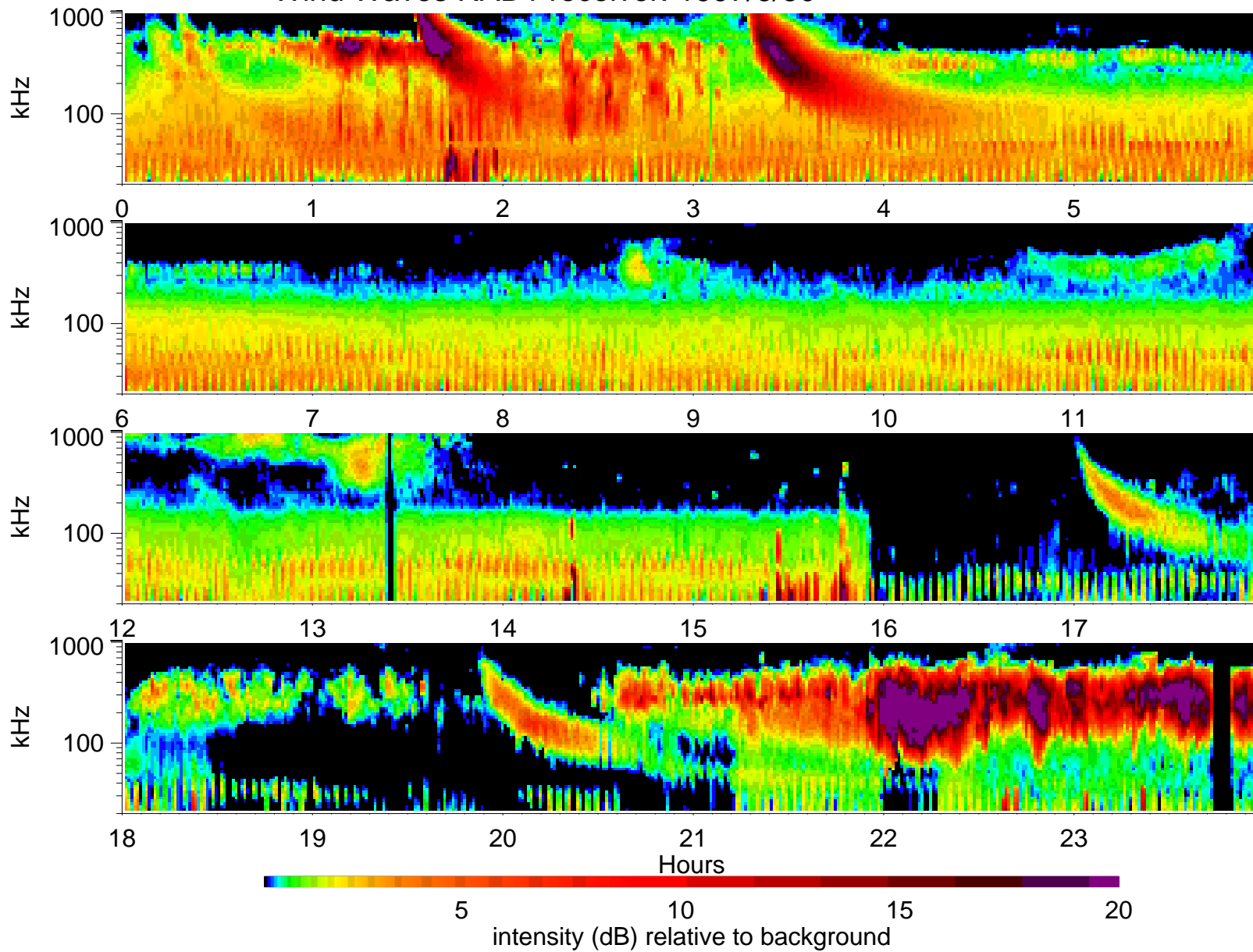
Wind Waves RAD1 receiver: 1997/6/30
