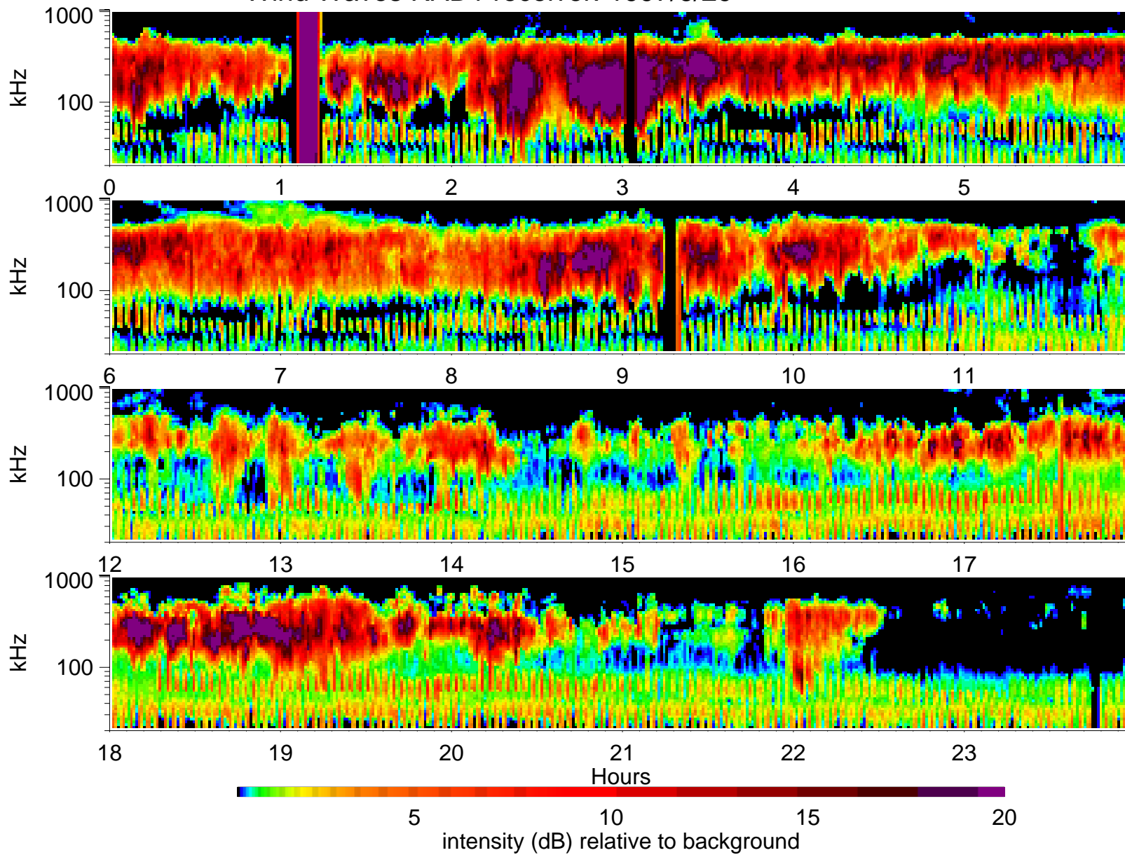
Wind Waves RAD1 receiver: 1997/6/29
