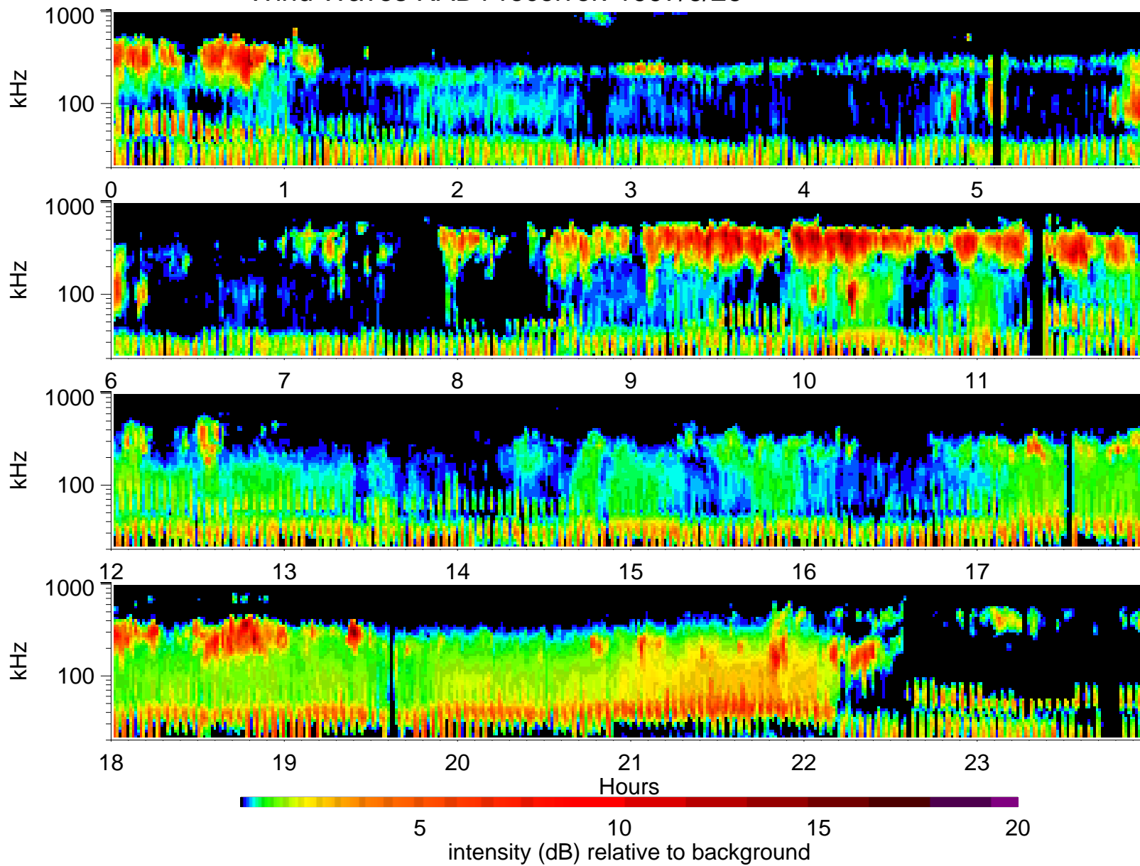
Wind Waves RAD1 receiver: 1997/6/26
