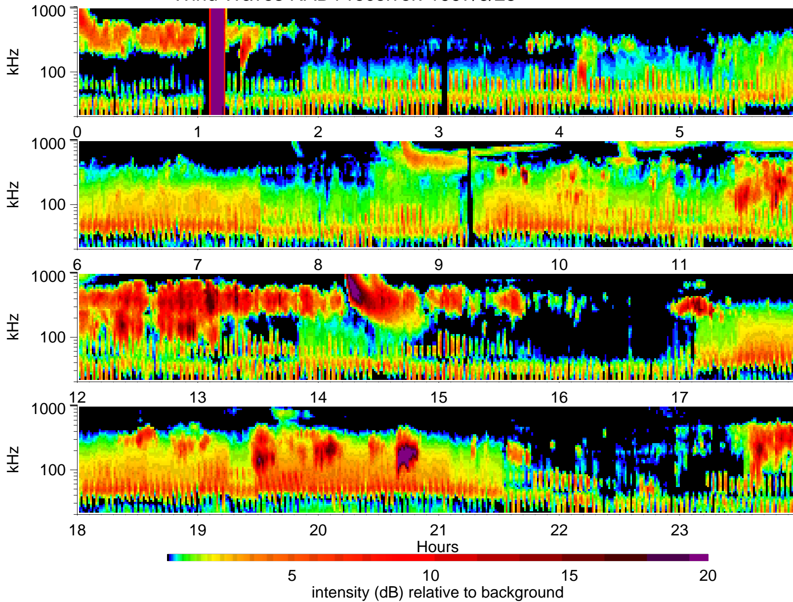
Wind Waves RAD1 receiver: 1997/6/25
