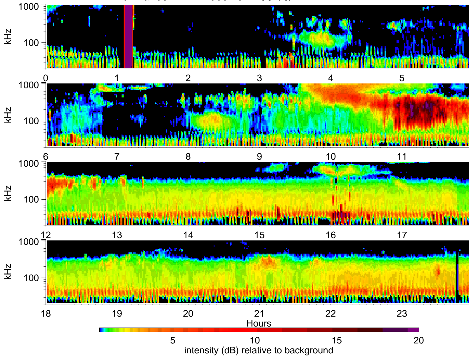
Wind Waves RAD1 receiver: 1997/6/21
