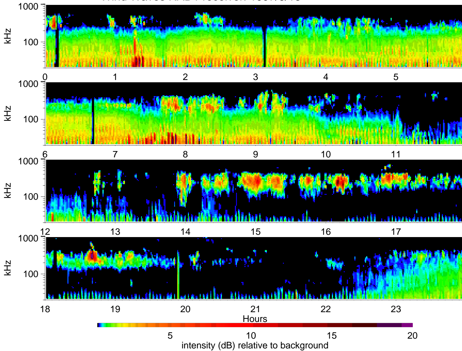
Wind Waves RAD1 receiver: 1997/6/18
