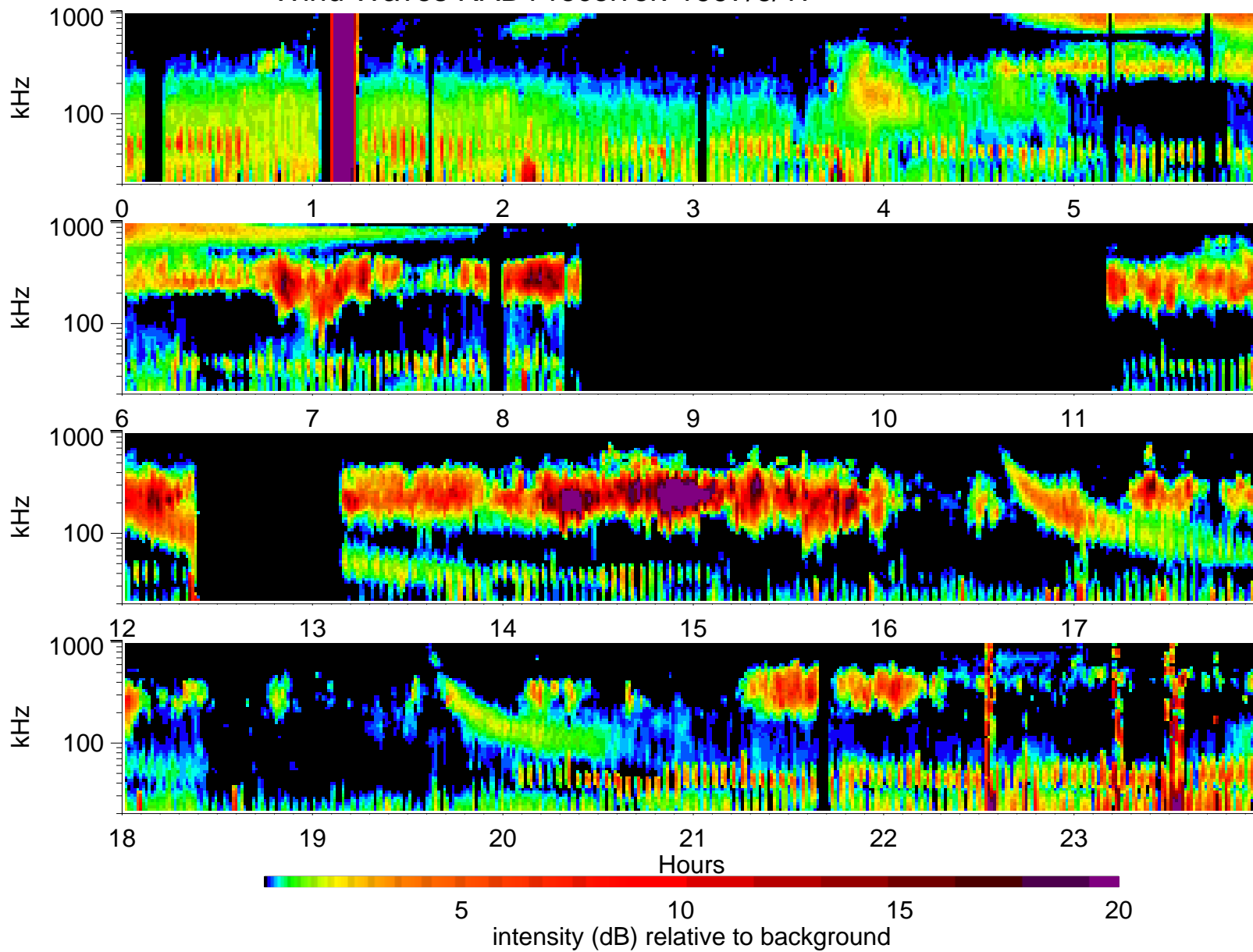
Wind Waves RAD1 receiver: 1997/6/17
