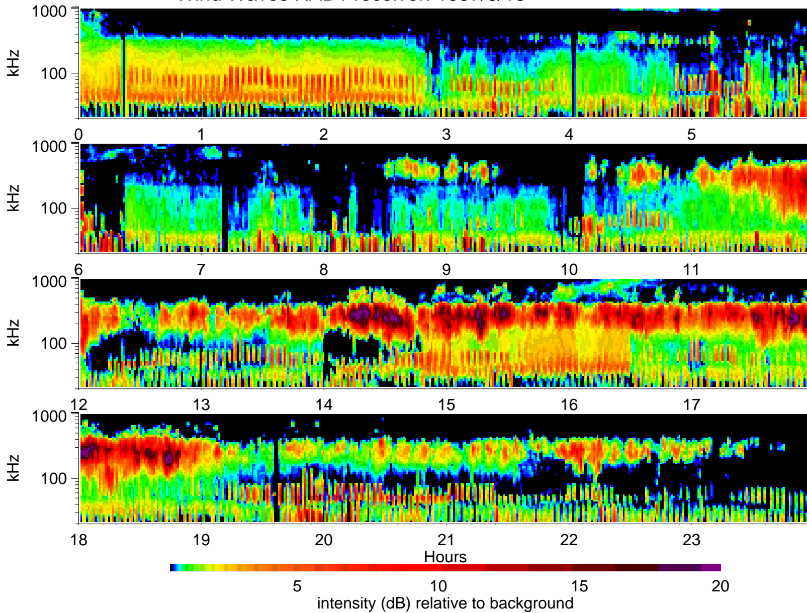
Wind Waves RAD1 receiver: 1997/6/16
