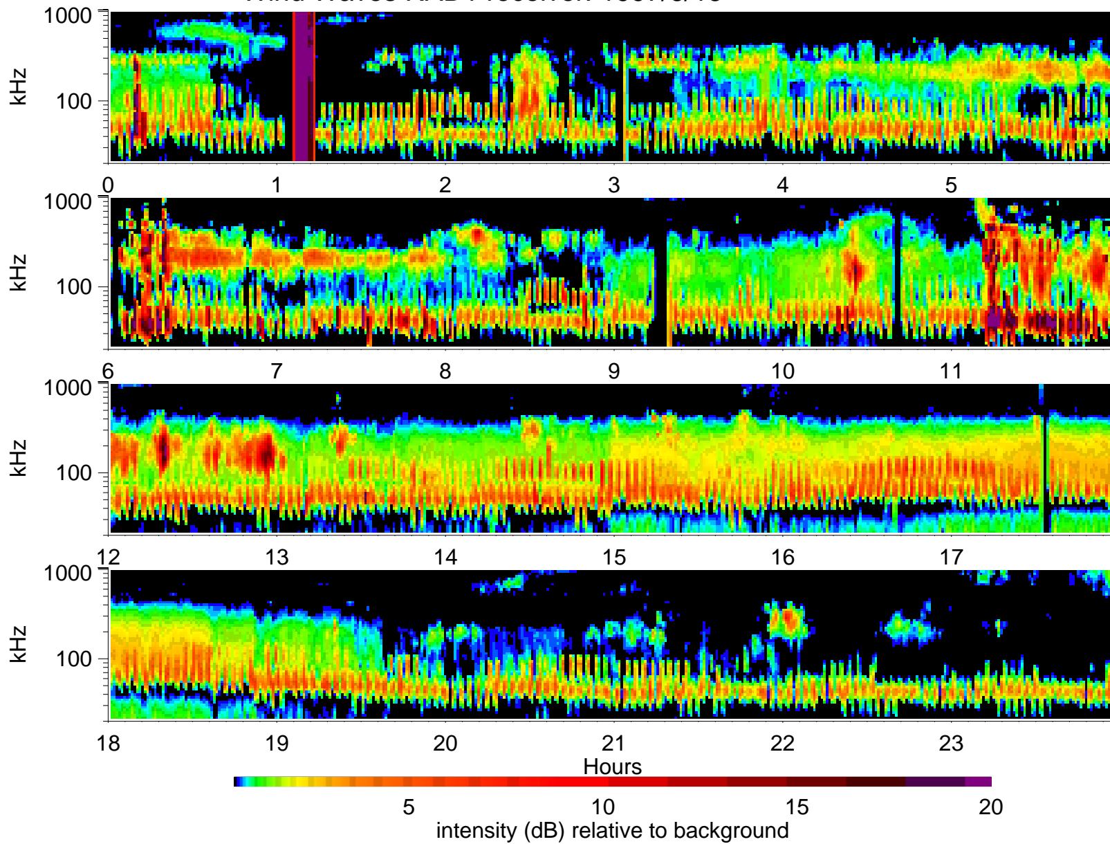
Wind Waves RAD1 receiver: 1997/6/15
