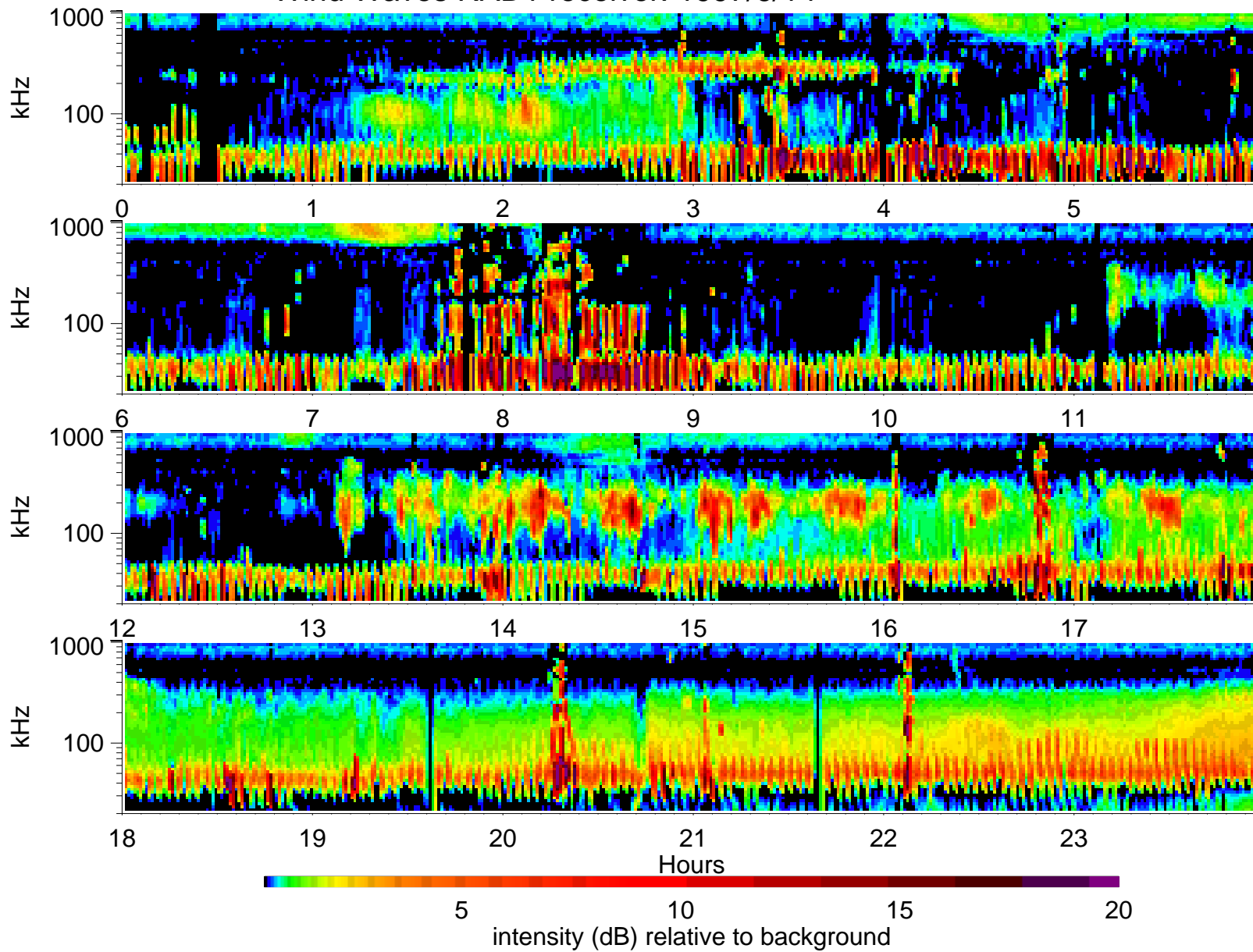
Wind Waves RAD1 receiver: 1997/6/14
