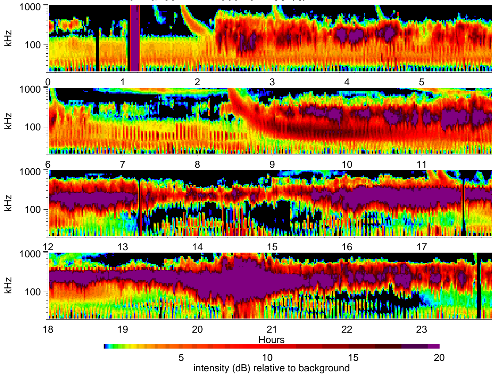
Wind Waves RAD1 receiver: 1997/6/7
