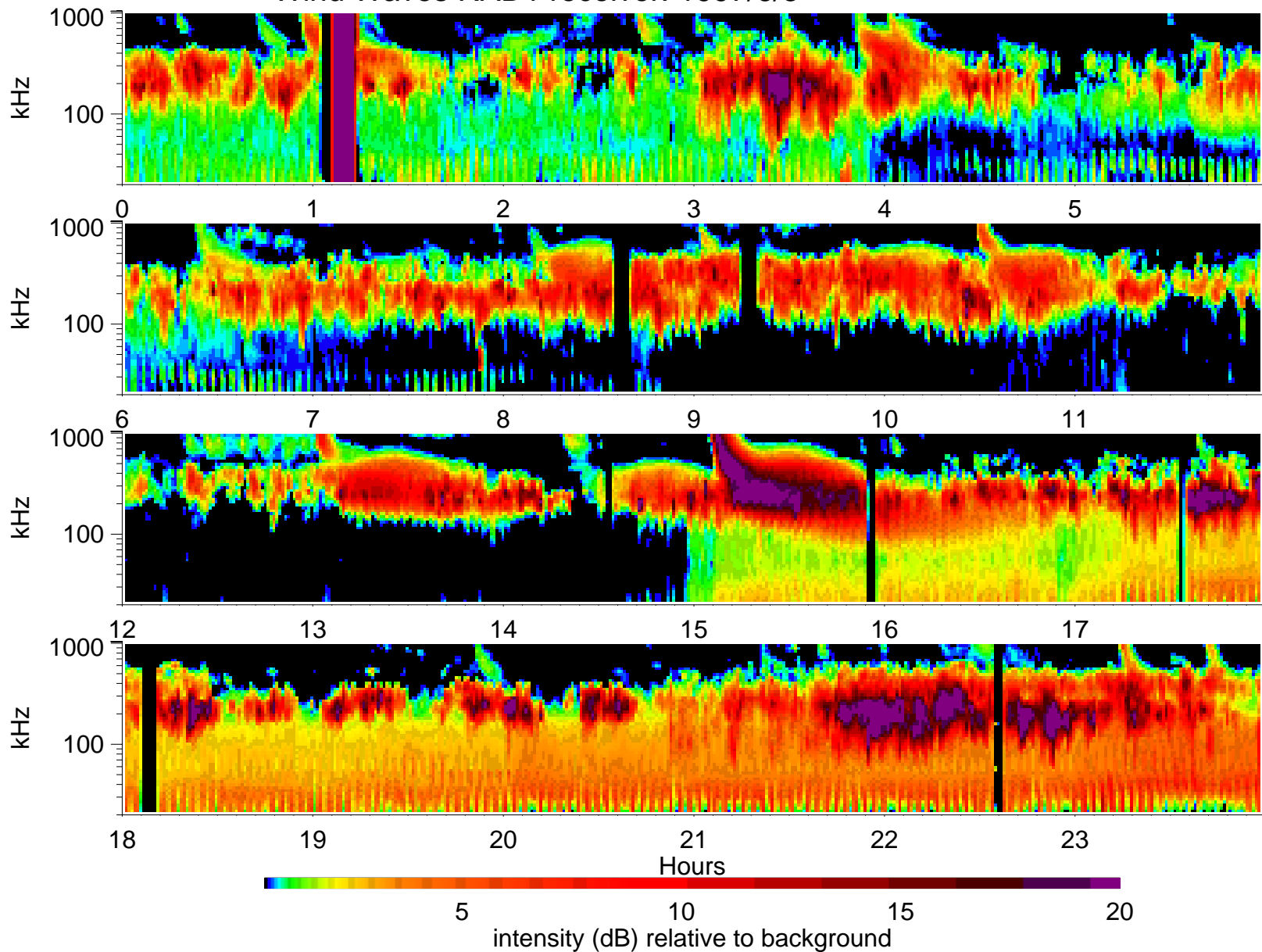
Wind Waves RAD1 receiver: 1997/6/5
