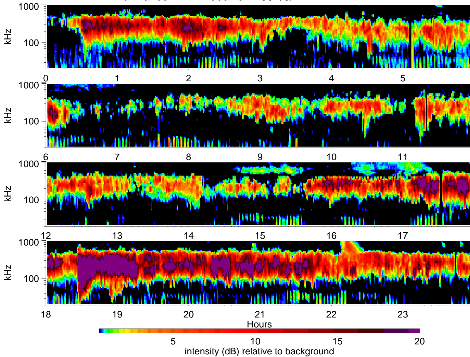
Wind Waves RAD1 receiver: 1997/6/4
