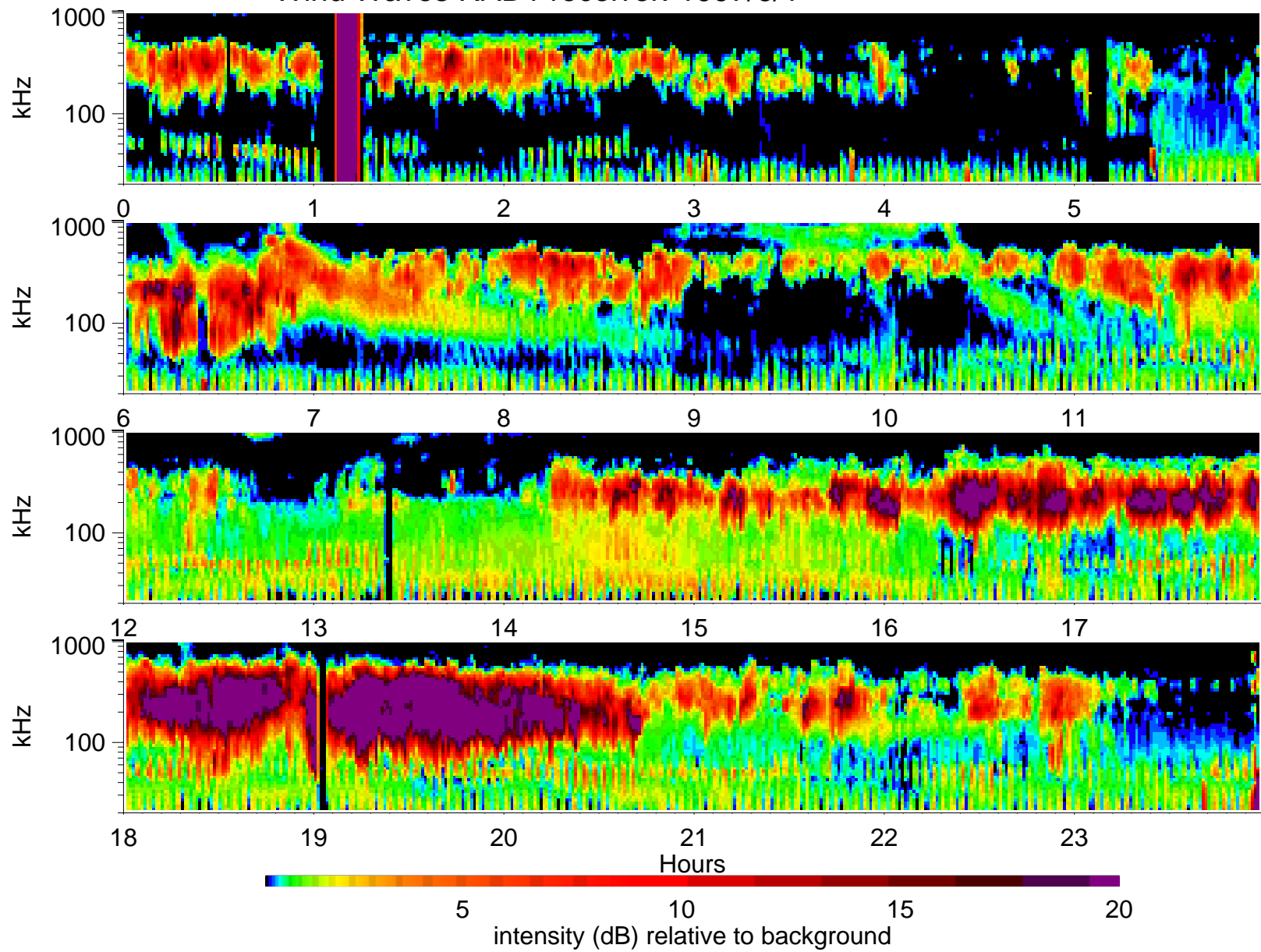
Wind Waves RAD1 receiver: 1997/6/1
